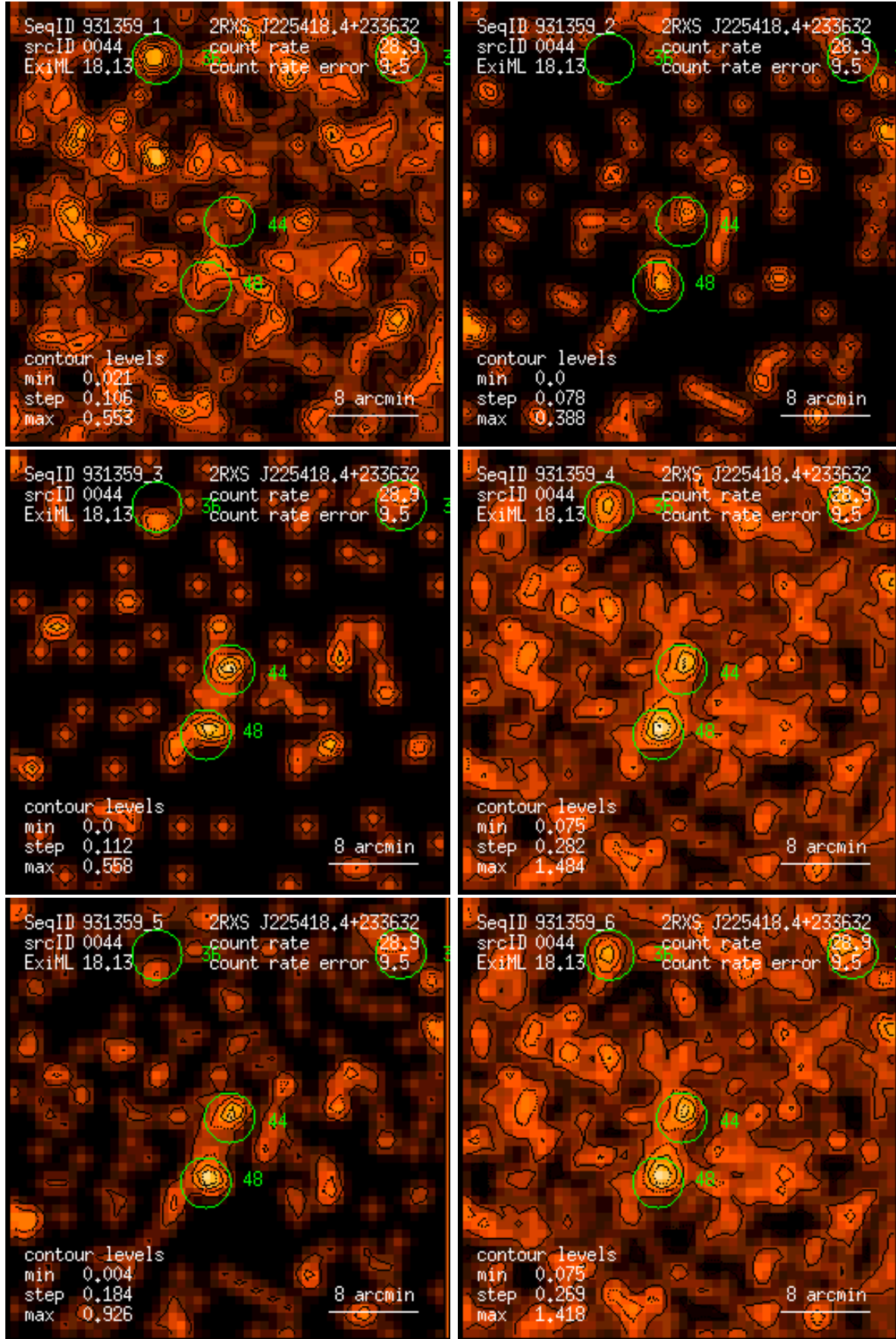
Figure 44: RASS 931359: detection 0044: band rate images, Gaussian filter: (1) PSPC channels 11 – 41, (2) 52 – 90, (3) 91 – 201, (4) 11 – 235, (5) 52 – 201, (6) 11 – 201. Broad band rates in counts/ks. Band rate contour levels in counts/ks/arcmin 2 .
