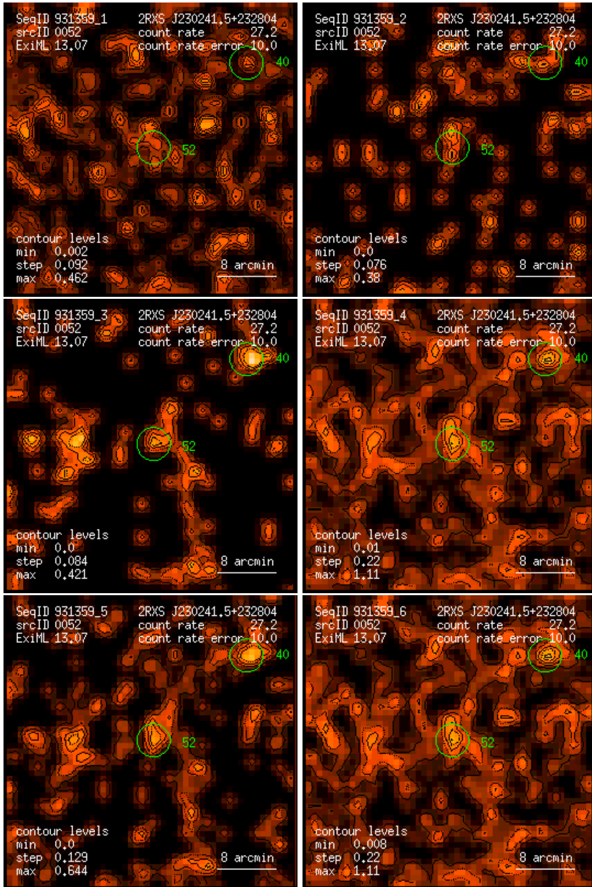
Figure 52: RASS 931359: detection 0052: band rate images, Gaussian filter: (1) PSPC channels 11 – 41, (2) 52 – 90, (3) 91 – 201, (4) 11 – 235, (5) 52 – 201, (6) 11 – 201. Broad band rates in counts/ks. Band rate contour levels in counts/ks/arcmin 2 .
