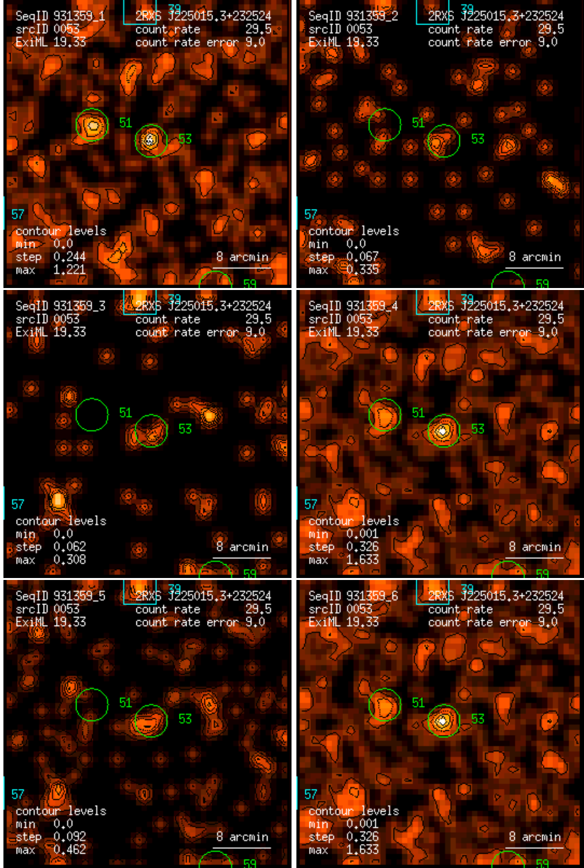
Figure 53: RASS 931359: detection 0053: band rate images, Gaussian filter: (1) PSPC channels 11 – 41, (2) 52 – 90, (3) 91 – 201, (4) 11 – 235, (5) 52 – 201, (6) 11 – 201. Broad band rates in counts/ks. Band rate contour levels in counts/ks/arcmin 2 .
