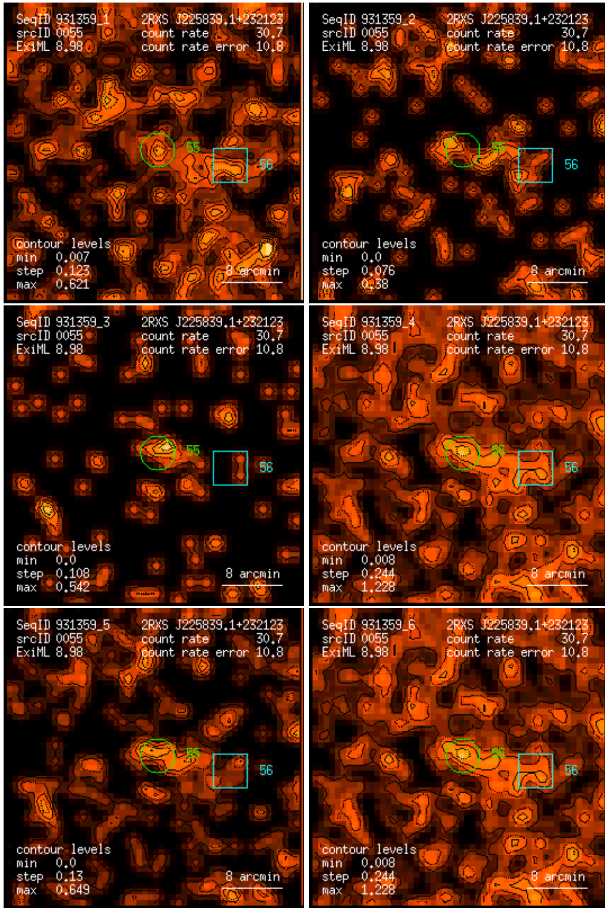
Figure 55: RASS 931359: detection 0055: band rate images, Gaussian filter: (1) PSPC channels 11 – 41, (2) 52 – 90, (3) 91 – 201, (4) 11 – 235, (5) 52 – 201, (6) 11 – 201. Broad band rates in counts/ks. Band rate contour levels in counts/ks/arcmin 2 .
