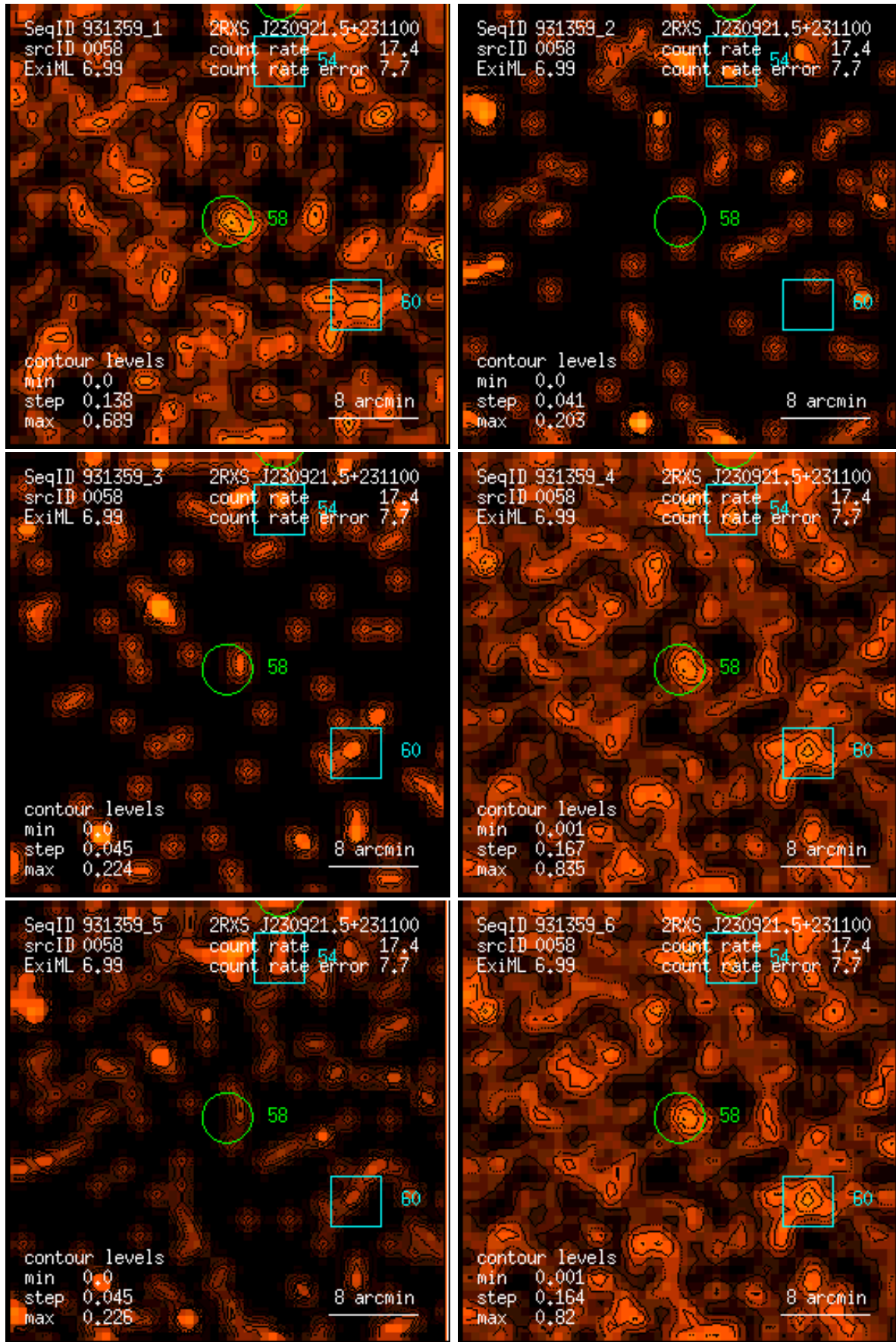
Figure 58: RASS 931359: detection 0058: band rate images, Gaussian filter: (1) PSPC channels 11 – 41, (2) 52 – 90, (3) 91 – 201, (4) 11 – 235, (5) 52 – 201, (6) 11 – 201. Broad band rates in counts/ks. Band rate contour levels in counts/ks/arcmin 2 .
