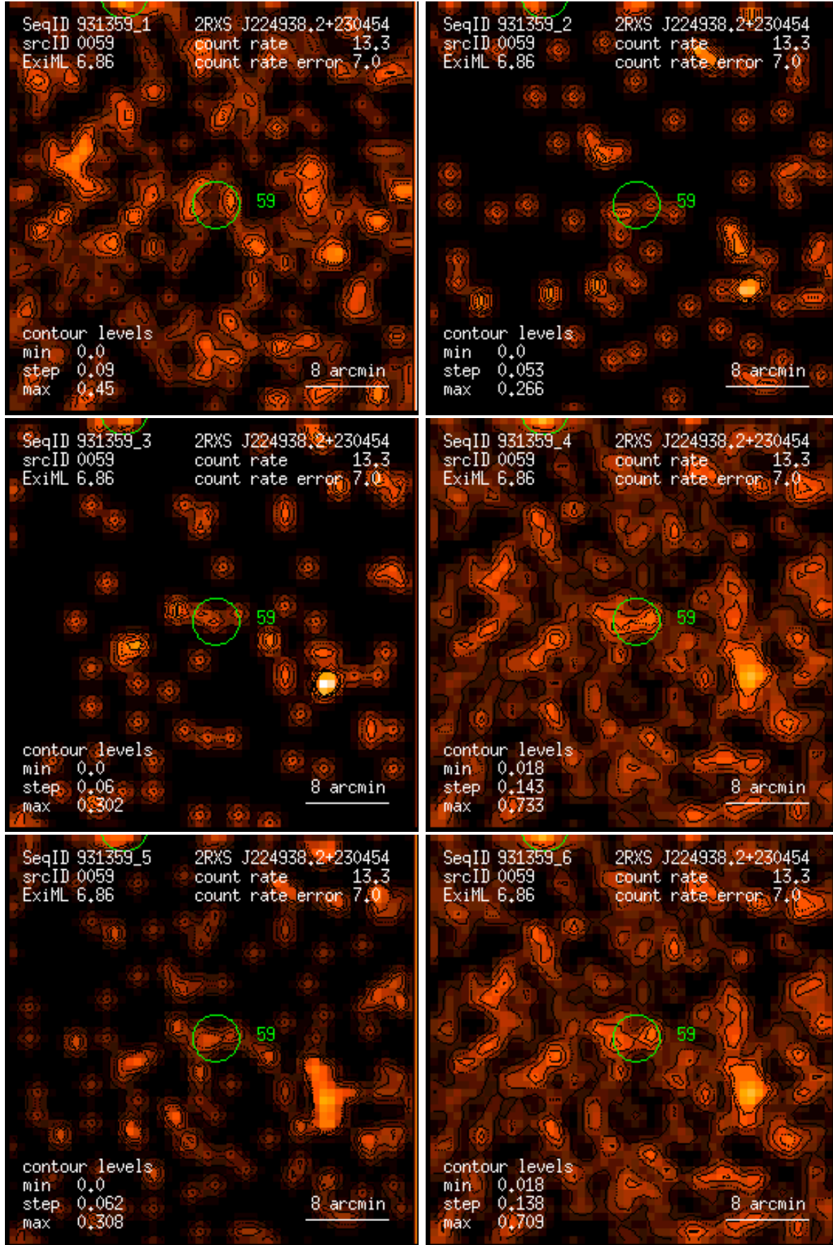
Figure 59: RASS 931359: detection 0059: band rate images, Gaussian filter: (1) PSPC channels 11 – 41, (2) 52 – 90, (3) 91 – 201, (4) 11 – 235, (5) 52 – 201, (6) 11 – 201. Broad band rates in counts/ks. Band rate contour levels in counts/ks/arcmin 2 .
