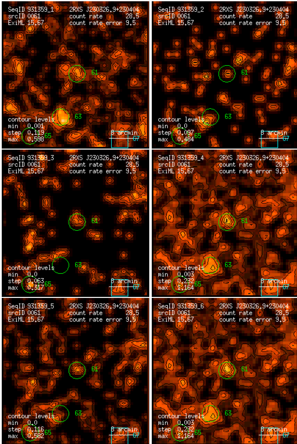
Figure 61: RASS 931359: detection 0061: band rate images, Gaussian filter: (1) PSPC channels 11 – 41, (2) 52 – 90, (3) 91 – 201, (4) 11 – 235, (5) 52 – 201, (6) 11 – 201. Broad band rates in counts/ks. Band rate contour levels in counts/ks/arcmin 2 .
