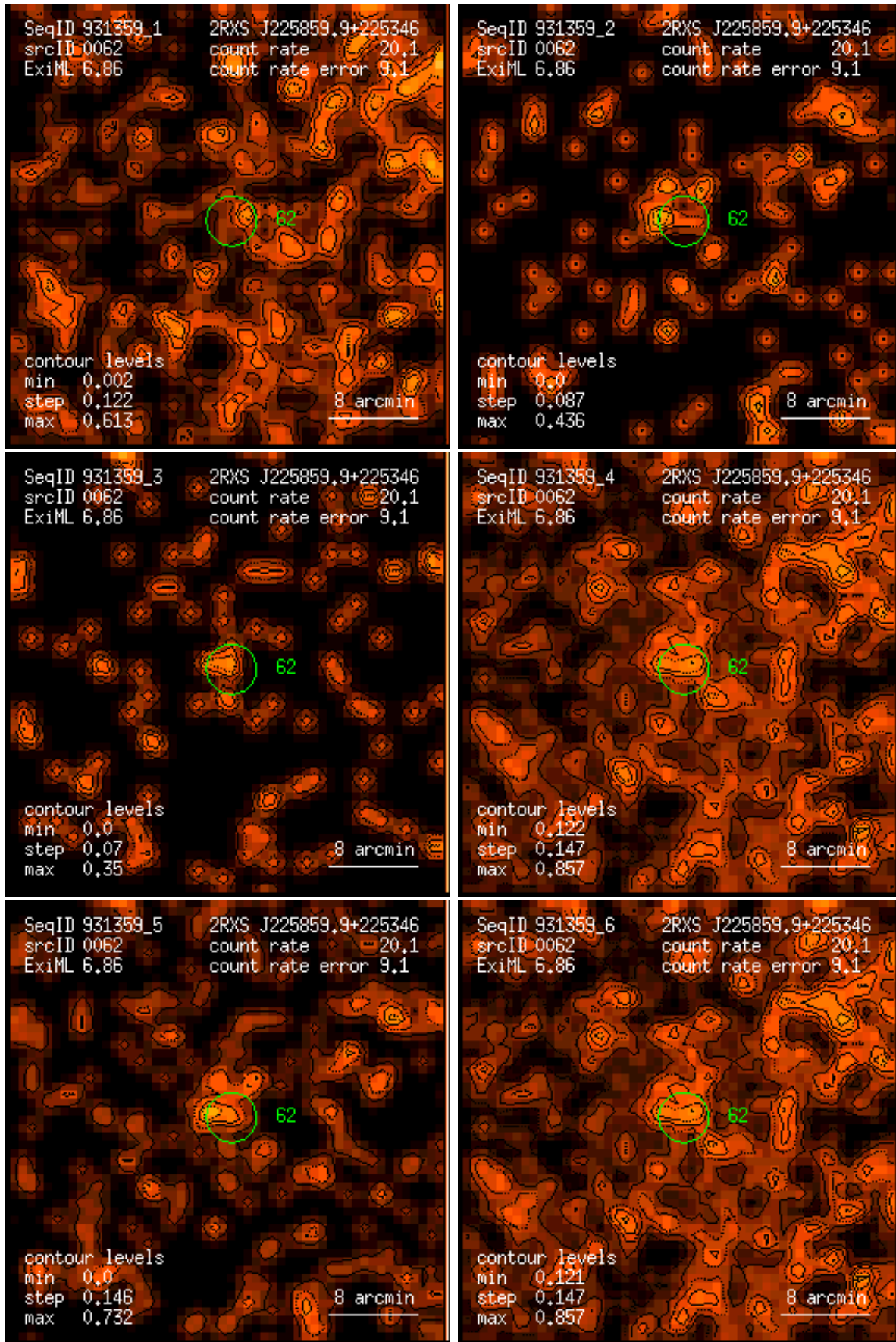
Figure 62: RASS 931359: detection 0062: band rate images, Gaussian filter: (1) PSPC channels 11 – 41, (2) 52 – 90, (3) 91 – 201, (4) 11 – 235, (5) 52 – 201, (6) 11 – 201. Broad band rates in counts/ks. Band rate contour levels in counts/ks/arcmin 2 .
