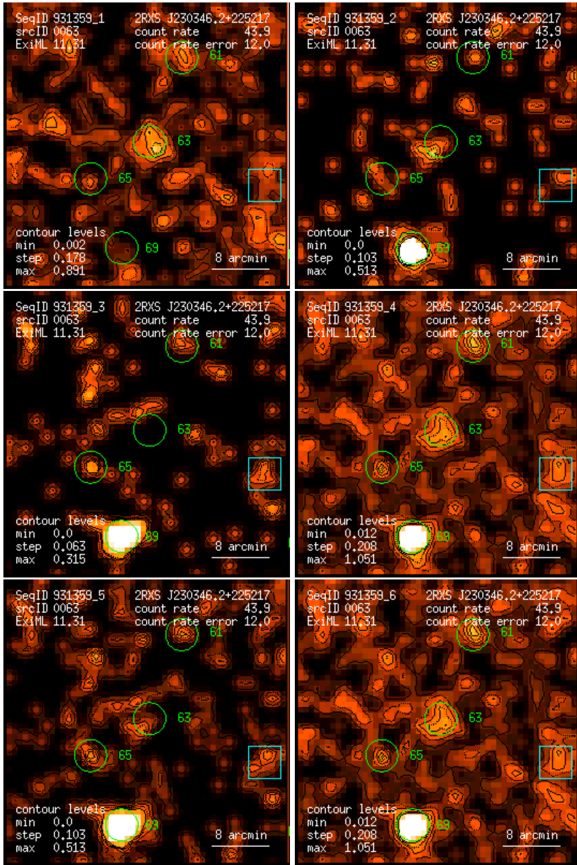
Figure 63: RASS 931359: detection 0063: band rate images, Gaussian filter: (1) PSPC channels 11 – 41, (2) 52 – 90, (3) 91 – 201, (4) 11 – 235, (5) 52 – 201, (6) 11 – 201. Broad band rates in counts/ks. Band rate contour levels in counts/ks/arcmin 2 .
