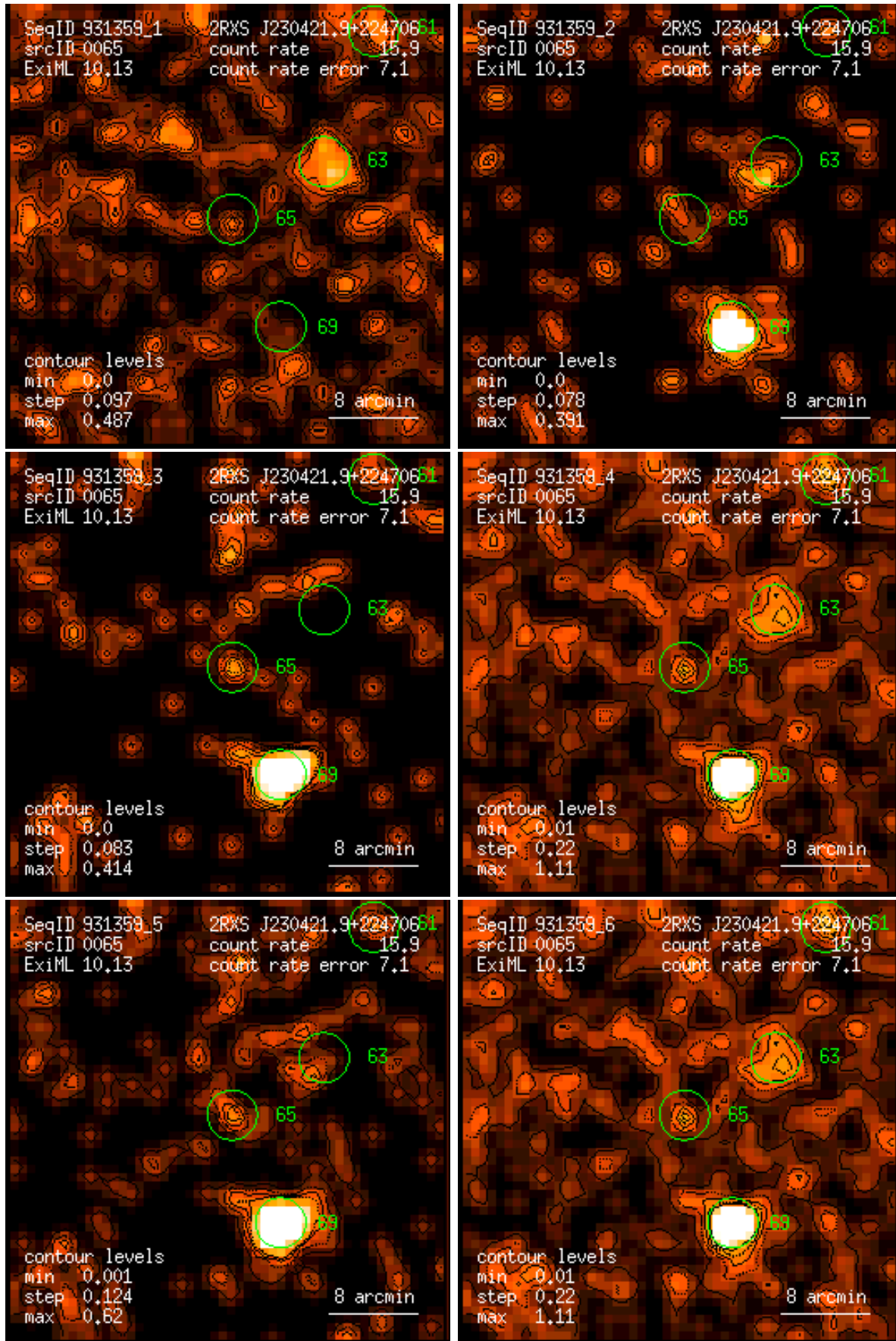
Figure 65: RASS 931359: detection 0065: band rate images, Gaussian filter: (1) PSPC channels 11 – 41, (2) 52 – 90, (3) 91 – 201, (4) 11 – 235, (5) 52 – 201, (6) 11 – 201. Broad band rates in counts/ks. Band rate contour levels in counts/ks/arcmin 2 .
