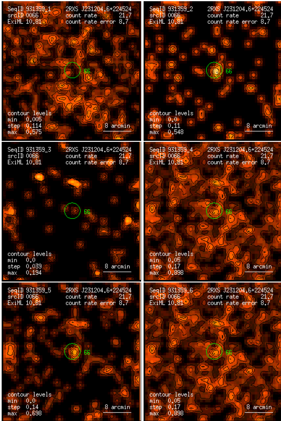
Figure 66: RASS 931359: detection 0066: band rate images, Gaussian filter: (1) PSPC channels 11 – 41, (2) 52 – 90, (3) 91 – 201, (4) 11 – 235, (5) 52 – 201, (6) 11 – 201. Broad band rates in counts/ks. Band rate contour levels in counts/ks/arcmin 2 .
