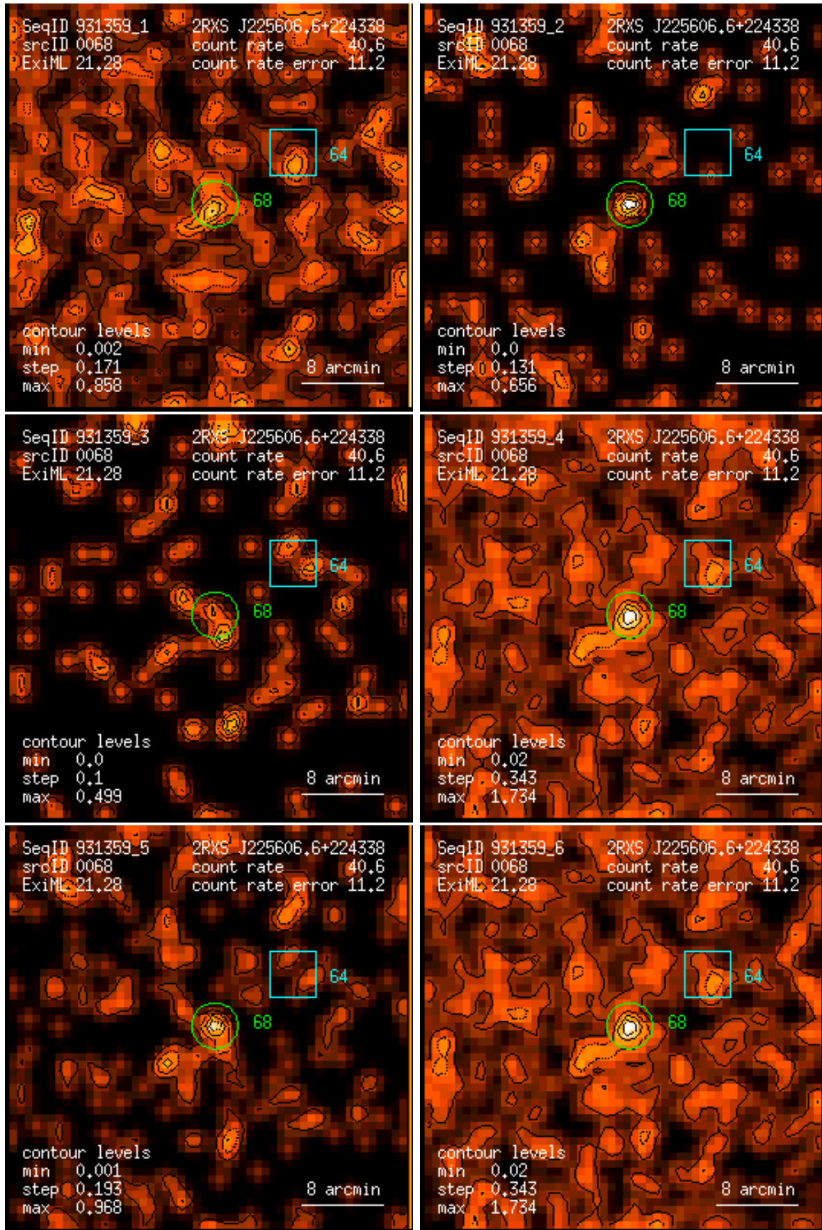
Figure 68: RASS 931359: detection 0068: band rate images, Gaussian filter: (1) PSPC channels 11 – 41, (2) 52 – 90, (3) 91 – 201, (4) 11 – 235, (5) 52 – 201, (6) 11 – 201. Broad band rates in counts/ks. Band rate contour levels in counts/ks/arcmin 2 .
