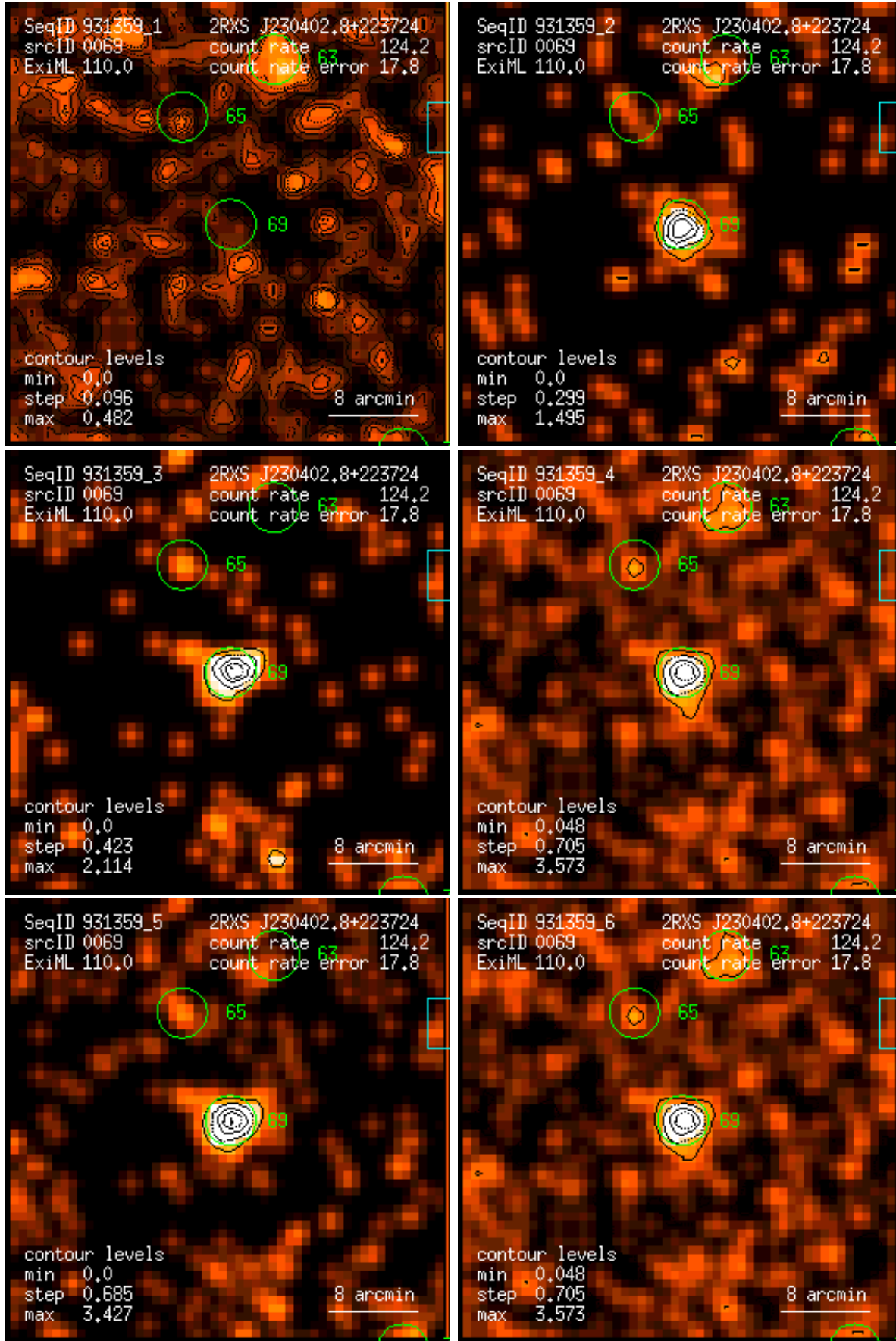
Figure 69: RASS 931359: detection 0069: band rate images, Gaussian filter: (1) PSPC channels 11 – 41, (2) 52 – 90, (3) 91 – 201, (4) 11 – 235, (5) 52 – 201, (6) 11 – 201. Broad band rates in counts/ks. Band rate contour levels in counts/ks/arcmin 2 .
