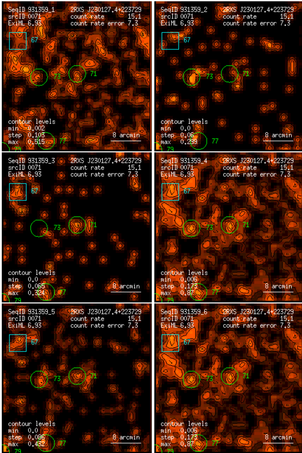
Figure 71: RASS 931359: detection 0071: band rate images, Gaussian filter: (1) PSPC channels 11 – 41, (2) 52 – 90, (3) 91 – 201, (4) 11 – 235, (5) 52 – 201, (6) 11 – 201. Broad band rates in counts/ks. Band rate contour levels in counts/ks/arcmin 2 .
