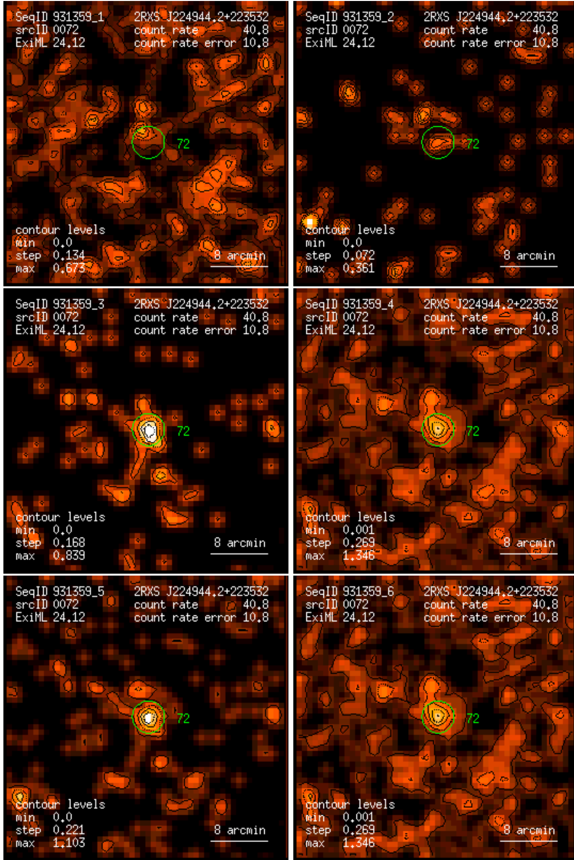
Figure 72: RASS 931359: detection 0072: band rate images, Gaussian filter: (1) PSPC channels 11 – 41, (2) 52 – 90, (3) 91 – 201, (4) 11 – 235, (5) 52 – 201, (6) 11 – 201. Broad band rates in counts/ks. Band rate contour levels in counts/ks/arcmin 2 .
