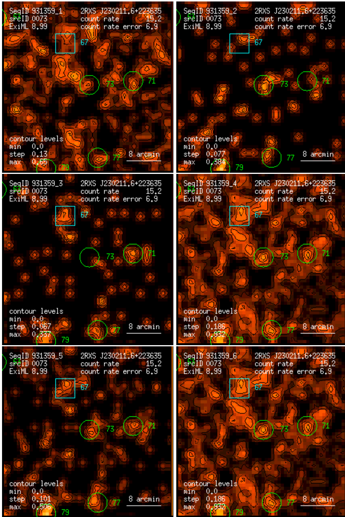
Figure 73: RASS 931359: detection 0073: band rate images, Gaussian filter: (1) PSPC channels 11 – 41, (2) 52 – 90, (3) 91 – 201, (4) 11 – 235, (5) 52 – 201, (6) 11 – 201. Broad band rates in counts/ks. Band rate contour levels in counts/ks/arcmin 2 .
