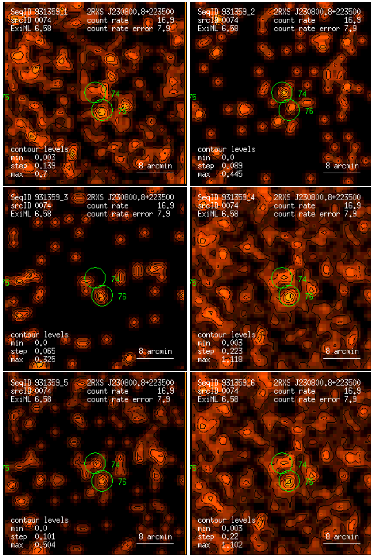
Figure 74: RASS 931359: detection 0074: band rate images, Gaussian filter: (1) PSPC channels 11 – 41, (2) 52 – 90, (3) 91 – 201, (4) 11 – 235, (5) 52 – 201, (6) 11 – 201. Broad band rates in counts/ks. Band rate contour levels in counts/ks/arcmin 2 .
