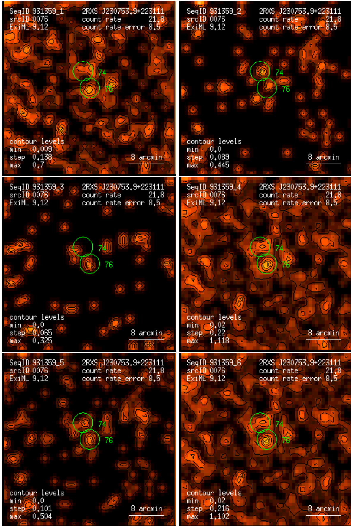
Figure 76: RASS 931359: detection 0076: band rate images, Gaussian filter: (1) PSPC channels 11 – 41, (2) 52 – 90, (3) 91 – 201, (4) 11 – 235, (5) 52 – 201, (6) 11 – 201. Broad band rates in counts/ks. Band rate contour levels in counts/ks/arcmin 2 .
