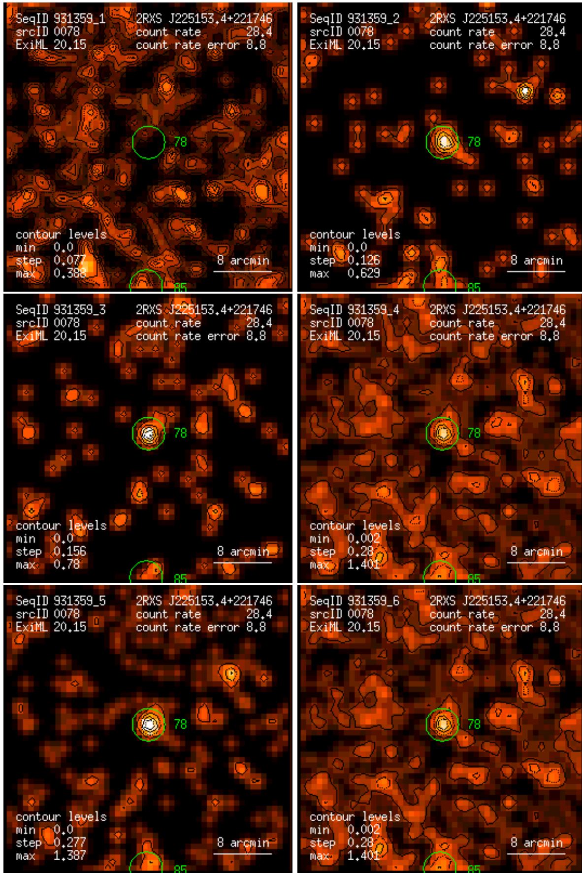
Figure 78: RASS 931359: detection 0078: band rate images, Gaussian filter: (1) PSPC channels 11 – 41, (2) 52 – 90, (3) 91 – 201, (4) 11 – 235, (5) 52 – 201, (6) 11 – 201. Broad band rates in counts/ks. Band rate contour levels in counts/ks/arcmin 2 .
