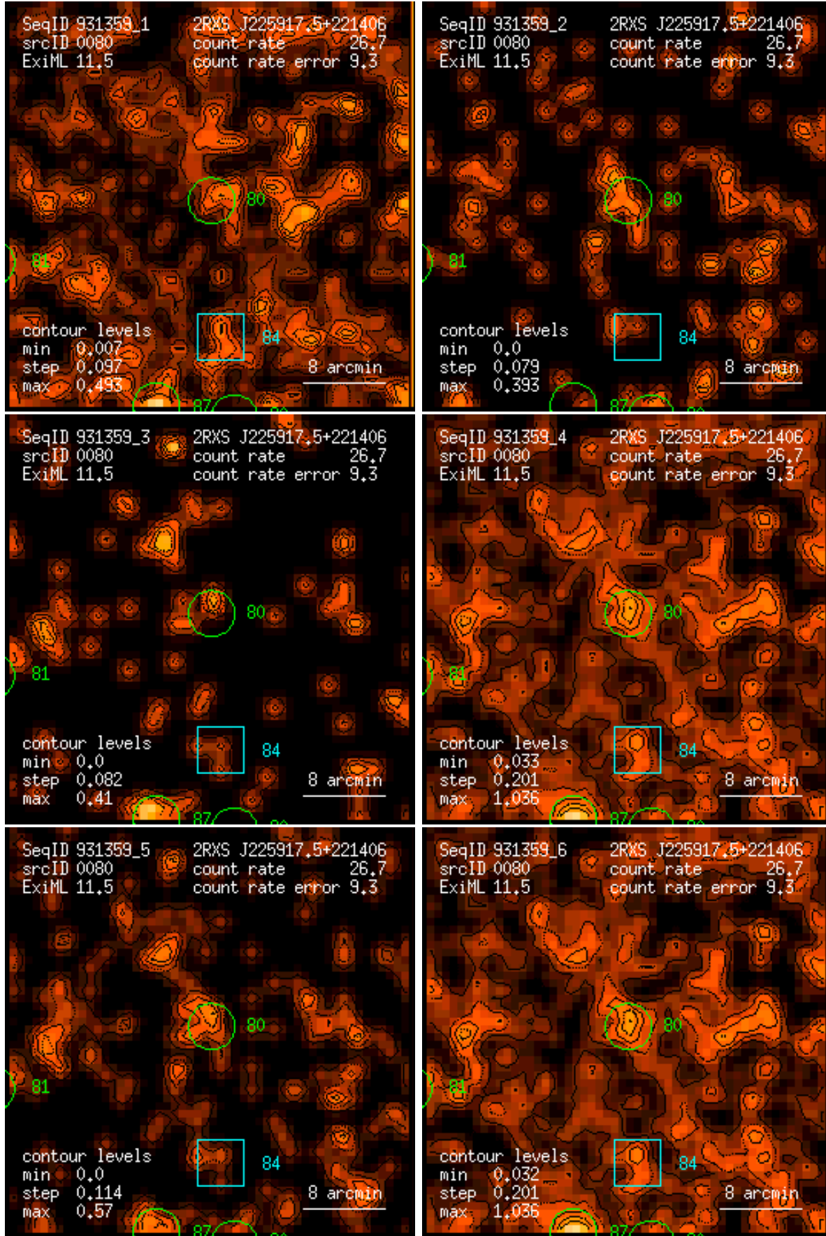
Figure 80: RASS 931359: detection 0080: band rate images, Gaussian filter: (1) PSPC channels 11 – 41, (2) 52 – 90, (3) 91 – 201, (4) 11 – 235, (5) 52 – 201, (6) 11 – 201. Broad band rates in counts/ks. Band rate contour levels in counts/ks/arcmin 2 .
