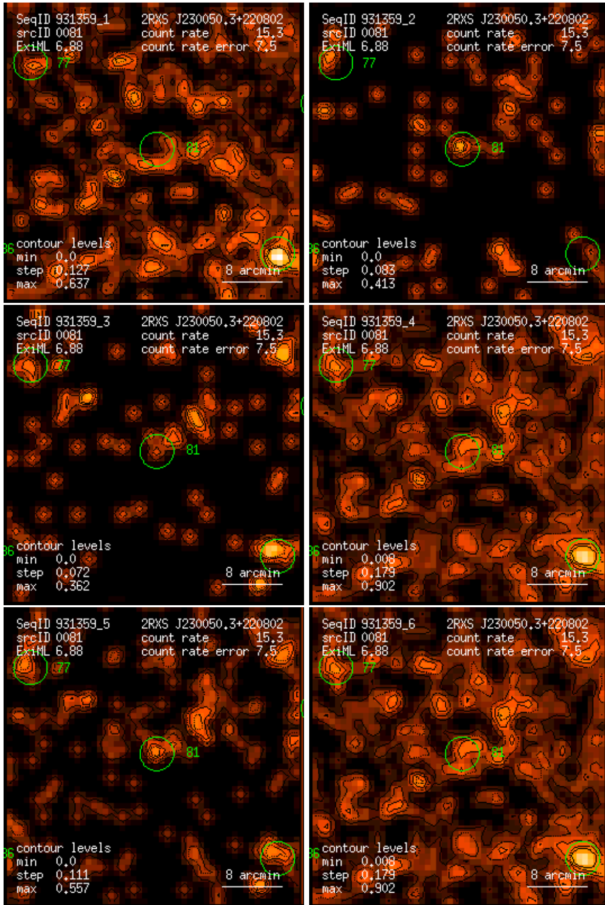
Figure 81: RASS 931359: detection 0081: band rate images, Gaussian filter: (1) PSPC channels 11 – 41, (2) 52 – 90, (3) 91 – 201, (4) 11 – 235, (5) 52 – 201, (6) 11 – 201. Broad band rates in counts/ks. Band rate contour levels in counts/ks/arcmin 2 .
