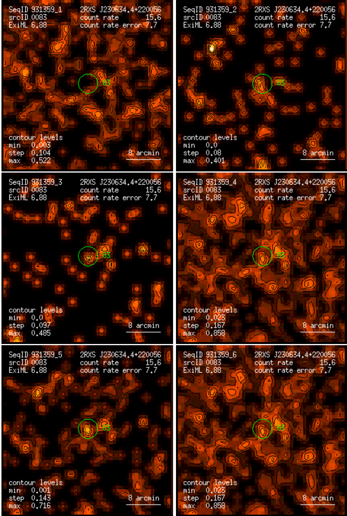
Figure 83: RASS 931359: detection 0083: band rate images, Gaussian filter: (1) PSPC channels 11 – 41, (2) 52 – 90, (3) 91 – 201, (4) 11 – 235, (5) 52 – 201, (6) 11 – 201. Broad band rates in counts/ks. Band rate contour levels in counts/ks/arcmin 2 .
