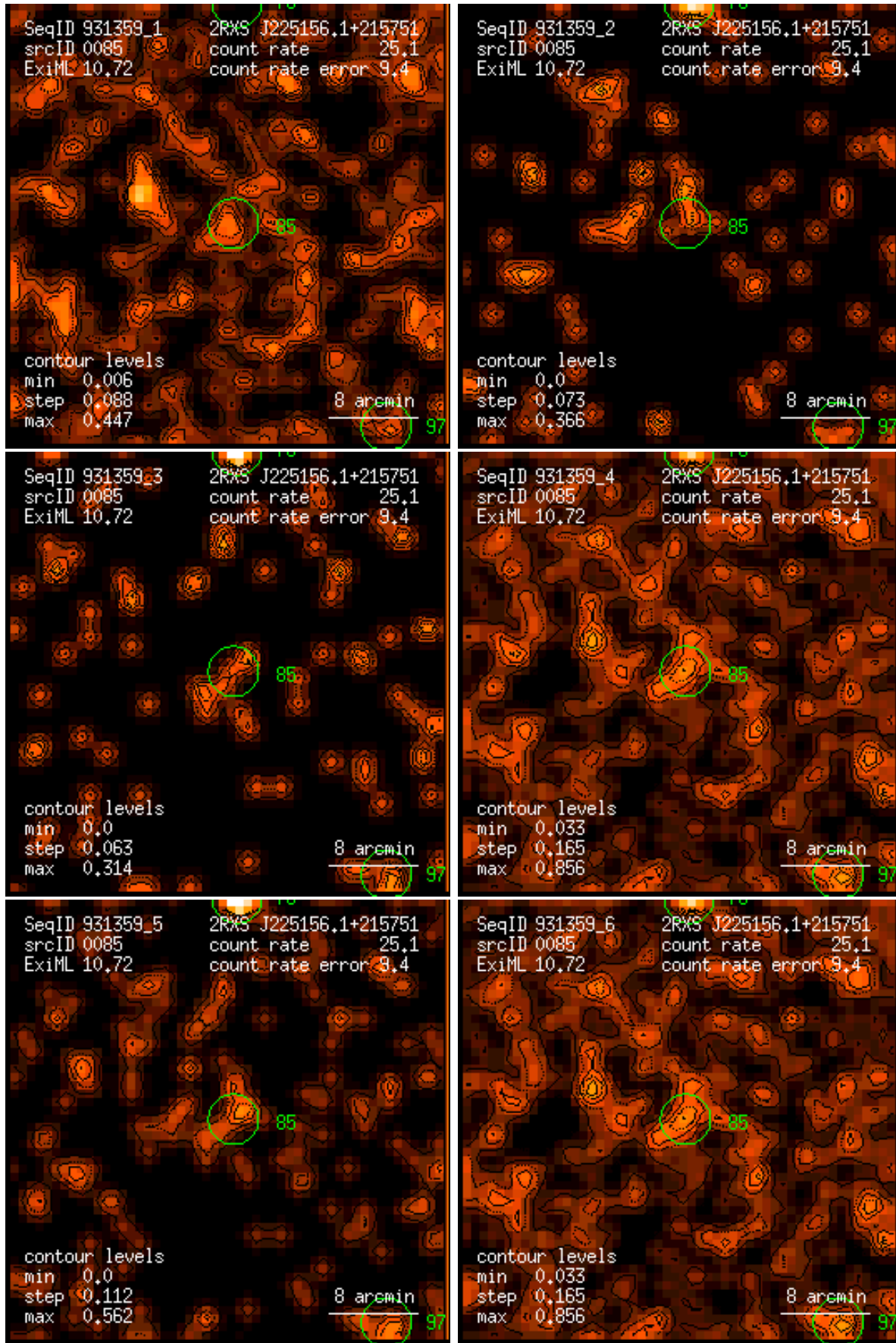
Figure 85: RASS 931359: detection 0085: band rate images, Gaussian filter: (1) PSPC channels 11 – 41, (2) 52 – 90, (3) 91 – 201, (4) 11 – 235, (5) 52 – 201, (6) 11 – 201. Broad band rates in counts/ks. Band rate contour levels in counts/ks/arcmin 2 .
