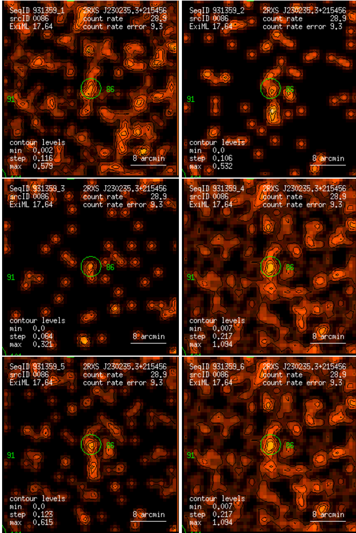
Figure 86: RASS 931359: detection 0086: band rate images, Gaussian filter: (1) PSPC channels 11 – 41, (2) 52 – 90, (3) 91 – 201, (4) 11 – 235, (5) 52 – 201, (6) 11 – 201. Broad band rates in counts/ks. Band rate contour levels in counts/ks/arcmin 2 .
