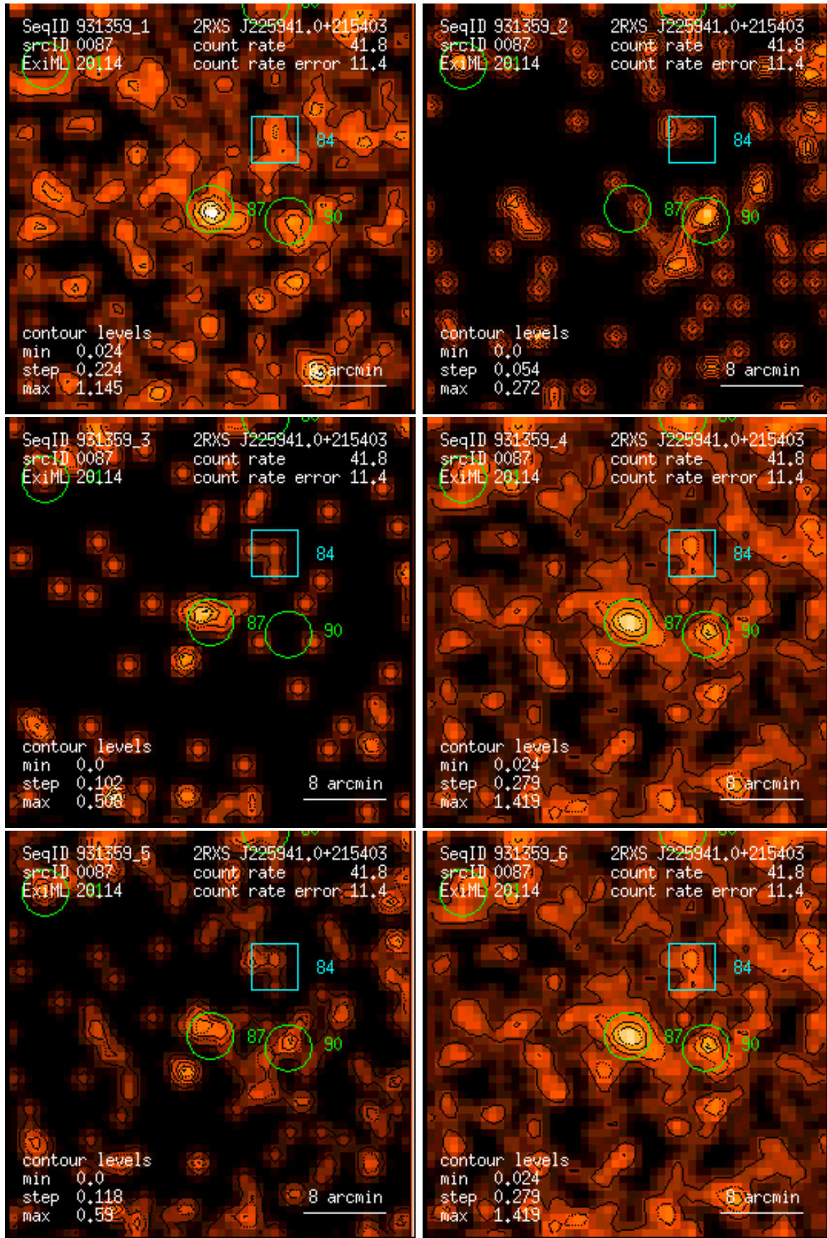
Figure 87: RASS 931359: detection 0087: band rate images, Gaussian filter: (1) PSPC channels 11 – 41, (2) 52 – 90, (3) 91 – 201, (4) 11 – 235, (5) 52 – 201, (6) 11 – 201. Broad band rates in counts/ks. Band rate contour levels in counts/ks/arcmin 2 .
