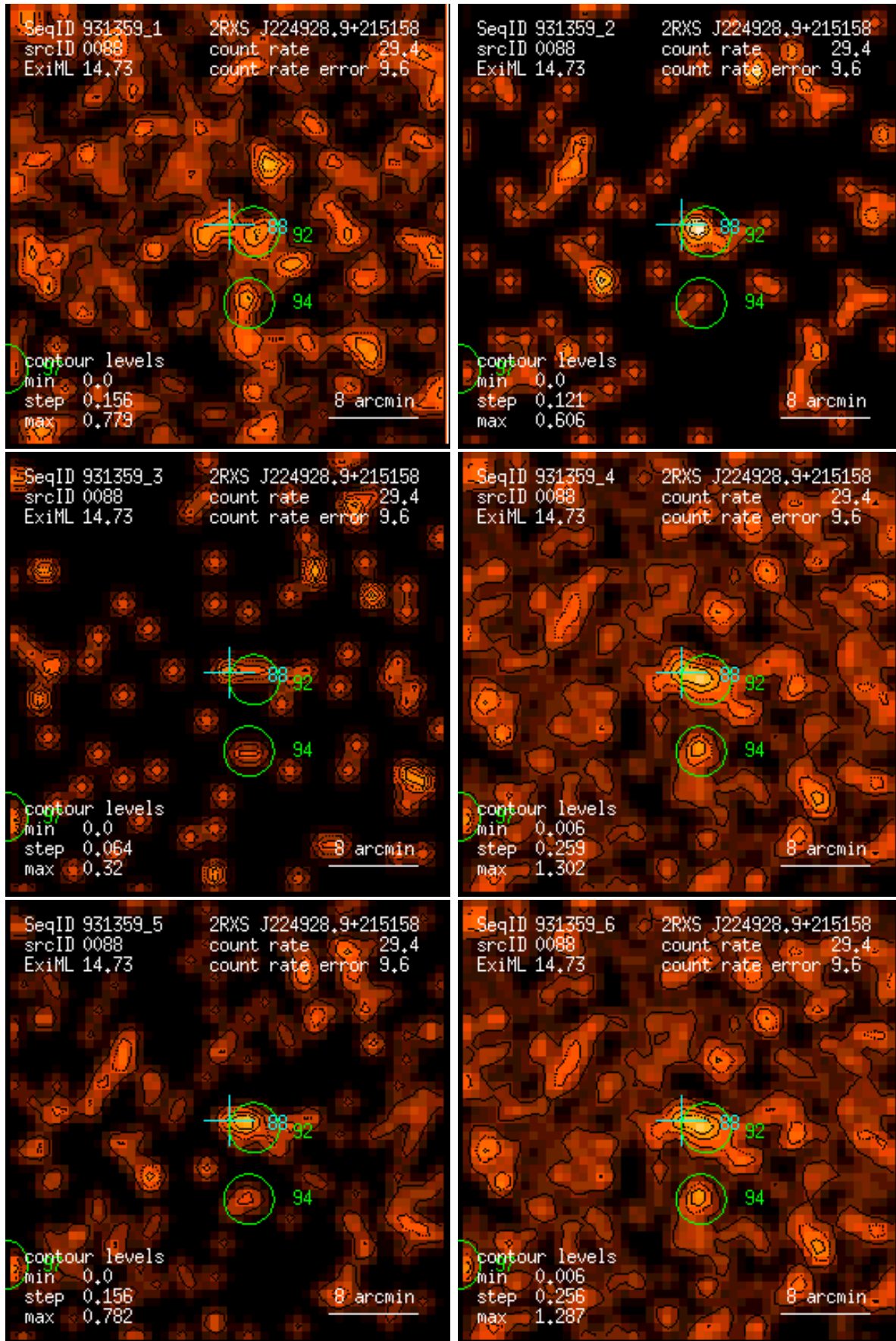
Figure 88: RASS 931359: detection 0088: band rate images, Gaussian filter: (1) PSPC channels 11 – 41, (2) 52 – 90, (3) 91 – 201, (4) 11 – 235, (5) 52 – 201, (6) 11 – 201. Broad band rates in counts/ks. Band rate contour levels in counts/ks/arcmin 2 .
