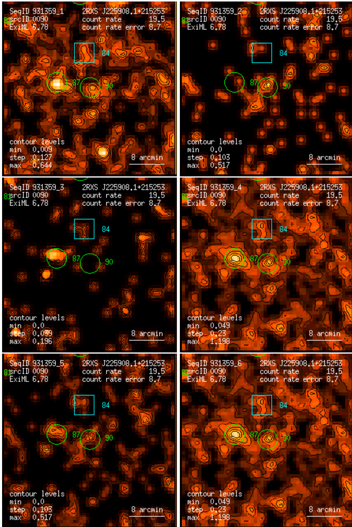
Figure 90: RASS 931359: detection 0090: band rate images, Gaussian filter: (1) PSPC channels 11 – 41, (2) 52 – 90, (3) 91 – 201, (4) 11 – 235, (5) 52 – 201, (6) 11 – 201. Broad band rates in counts/ks. Band rate contour levels in counts/ks/arcmin 2 .
