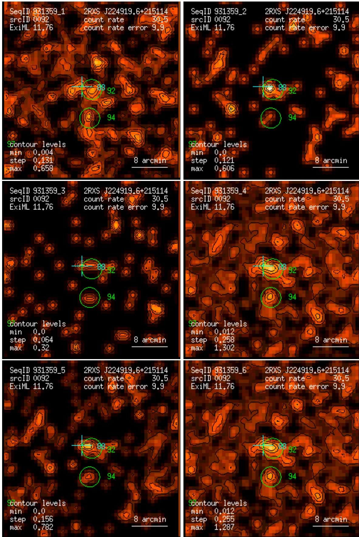
Figure 92: RASS 931359: detection 0092: band rate images, Gaussian filter: (1) PSPC channels 11 – 41, (2) 52 – 90, (3) 91 – 201, (4) 11 – 235, (5) 52 – 201, (6) 11 – 201. Broad band rates in counts/ks. Band rate contour levels in counts/ks/arcmin 2 .
