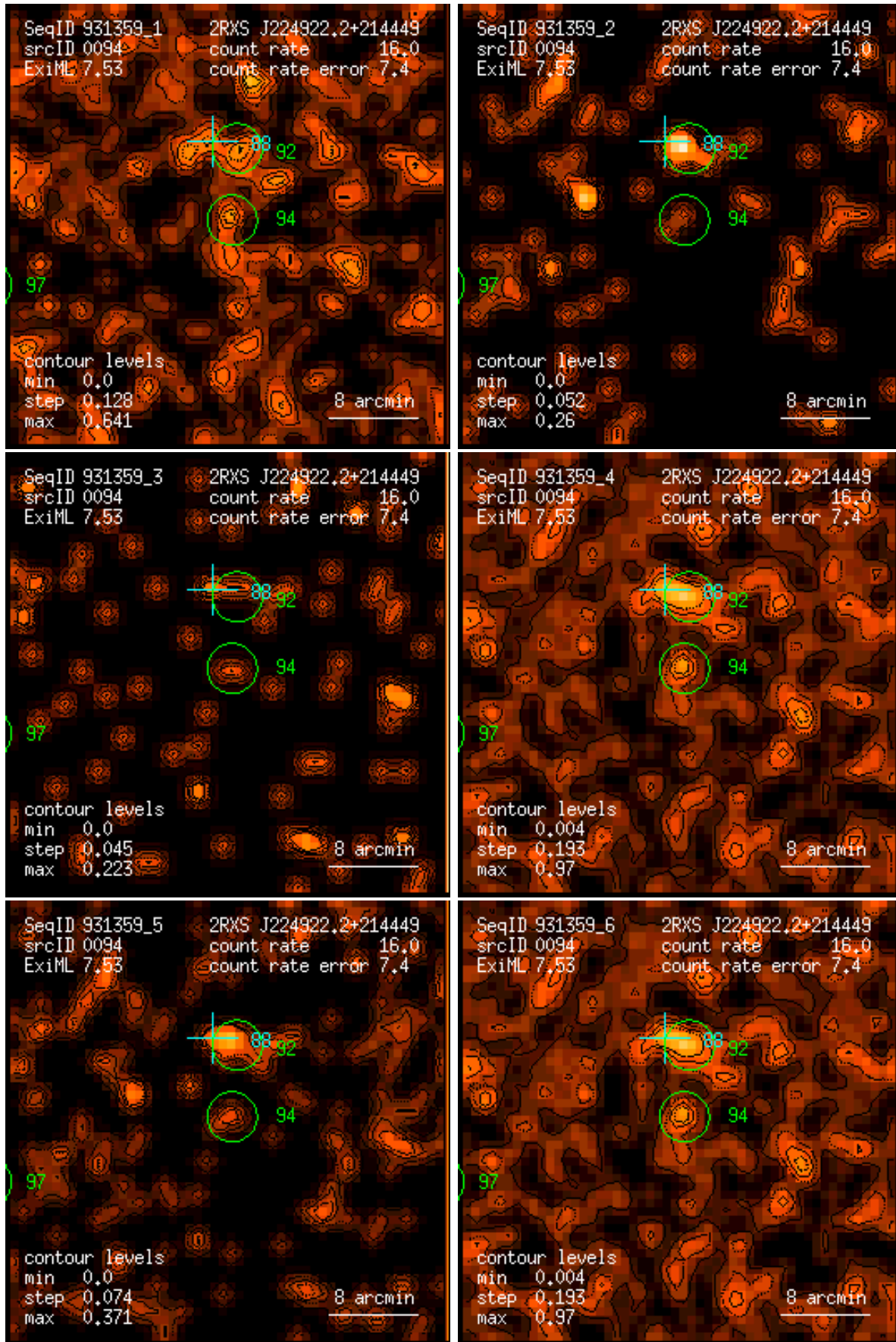
Figure 94: RASS 931359: detection 0094: band rate images, Gaussian filter: (1) PSPC channels 11 – 41, (2) 52 – 90, (3) 91 – 201, (4) 11 – 235, (5) 52 – 201, (6) 11 – 201. Broad band rates in counts/ks. Band rate contour levels in counts/ks/arcmin 2 .
