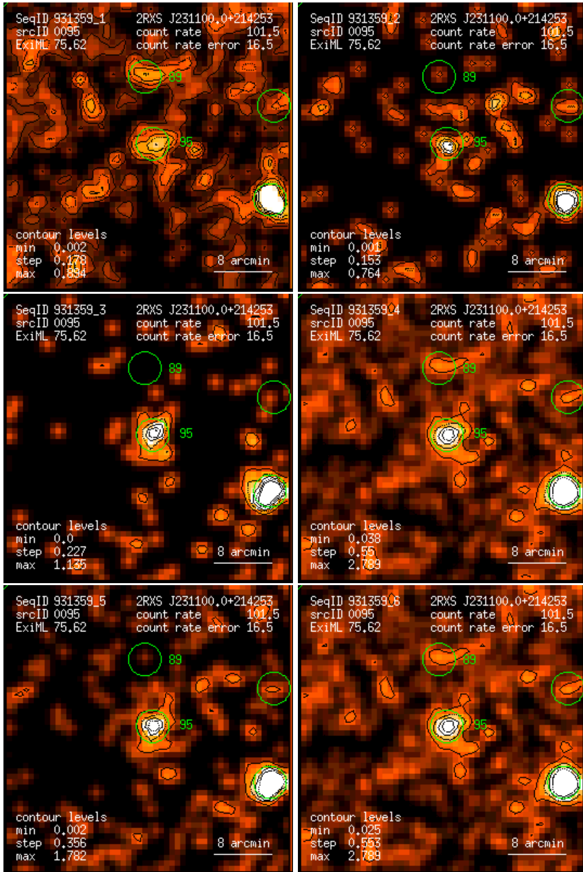
Figure 95: RASS 931359: detection 0095: band rate images, Gaussian filter: (1) PSPC channels 11 – 41, (2) 52 – 90, (3) 91 – 201, (4) 11 – 235, (5) 52 – 201, (6) 11 – 201. Broad band rates in counts/ks. Band rate contour levels in counts/ks/arcmin 2 .
