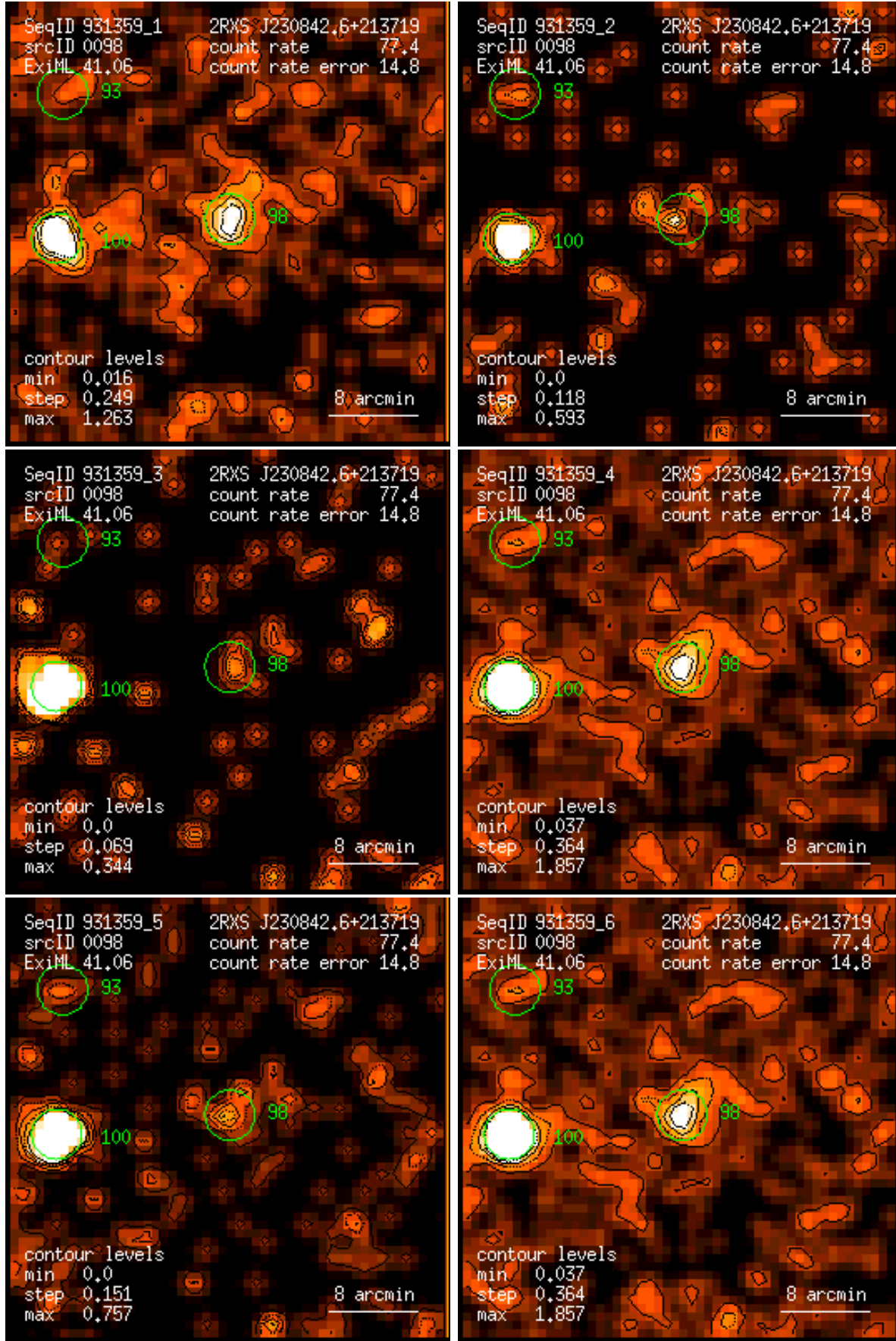
Figure 98: RASS 931359: detection 0098: band rate images, Gaussian filter: (1) PSPC channels 11 – 41, (2) 52 – 90, (3) 91 – 201, (4) 11 – 235, (5) 52 – 201, (6) 11 – 201. Broad band rates in counts/ks. Band rate contour levels in counts/ks/arcmin 2 .
