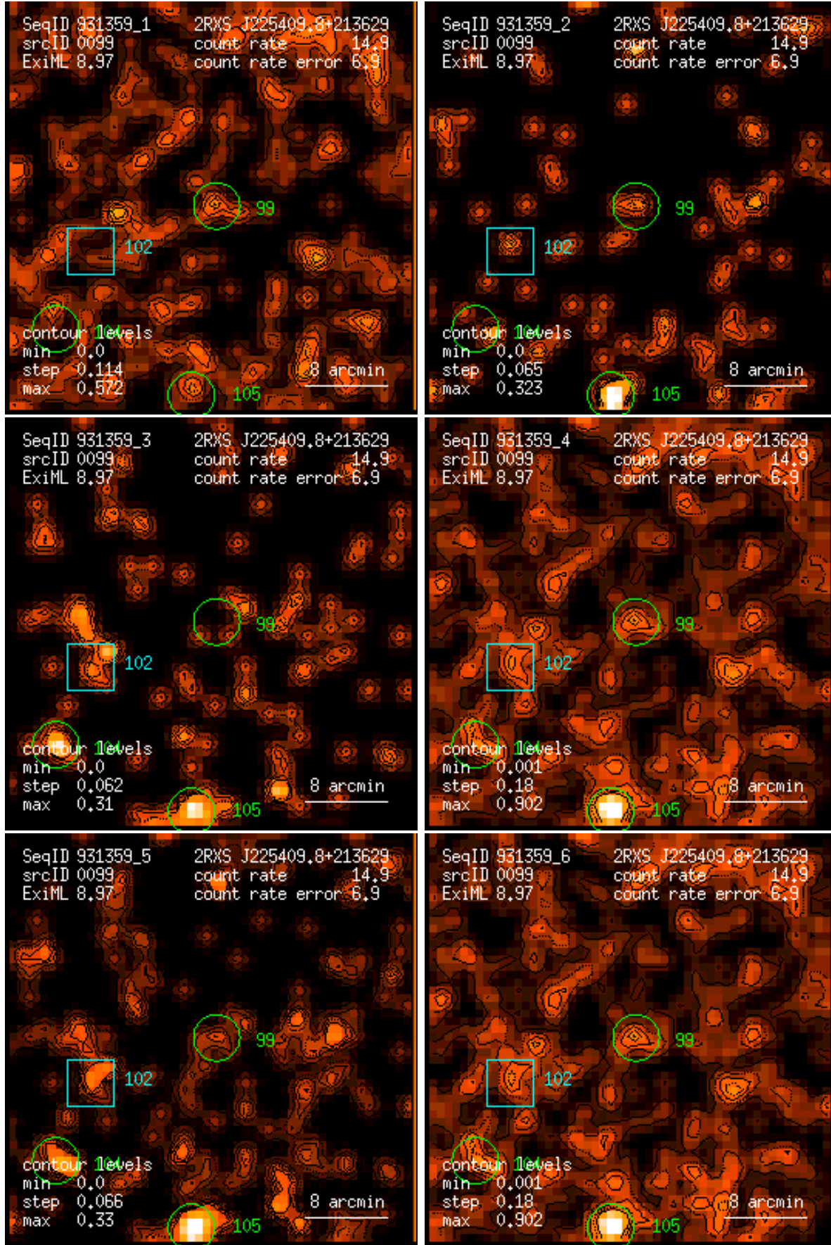
Figure 99: RASS 931359: detection 0099: band rate images, Gaussian filter: (1) PSPC channels 11 – 41, (2) 52 – 90, (3) 91 – 201, (4) 11 – 235, (5) 52 – 201, (6) 11 – 201. Broad band rates in counts/ks. Band rate contour levels in counts/ks/arcmin 2 .
