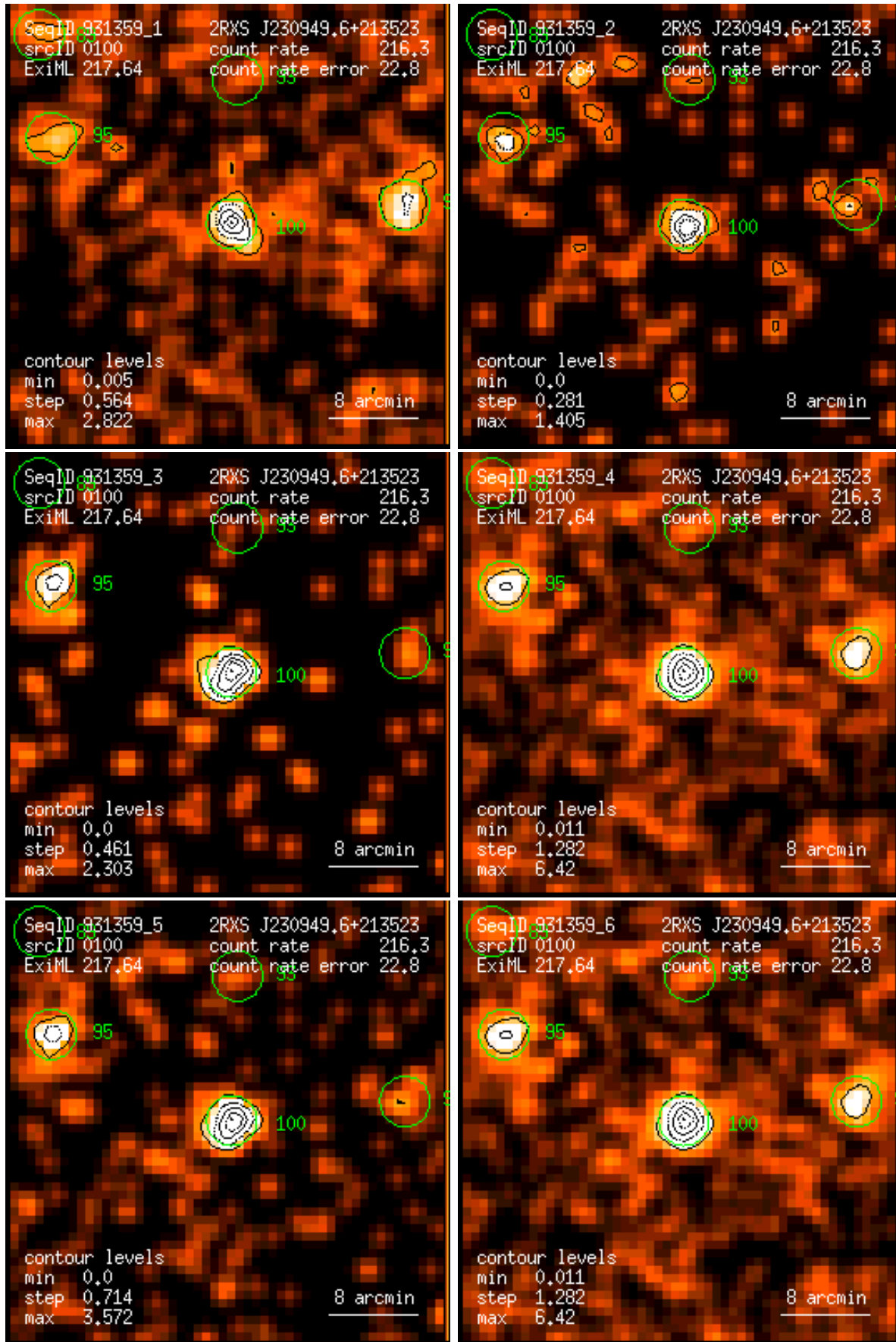
Figure 100: RASS 931359: detection 0100: band rate images, Gaussian filter: (1) PSPC channels 11 – 41, (2) 52 – 90, (3) 91 – 201, (4) 11 – 235, (5) 52 – 201, (6) 11 – 201. Broad band rates in counts/ks. Band rate contour levels in counts/ks/arcmin 2 .
