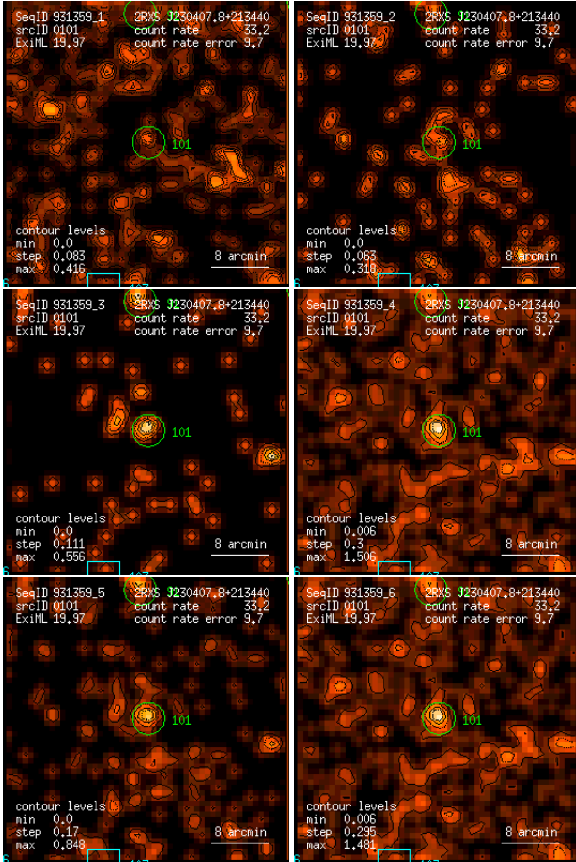
Figure 101: RASS 931359: detection 0101: band rate images, Gaussian filter: (1) PSPC channels 11 – 41, (2) 52 – 90, (3) 91 – 201, (4) 11 – 235, (5) 52 – 201, (6) 11 – 201. Broad band rates in counts/ks. Band rate contour levels in counts/ks/arcmin 2 .
