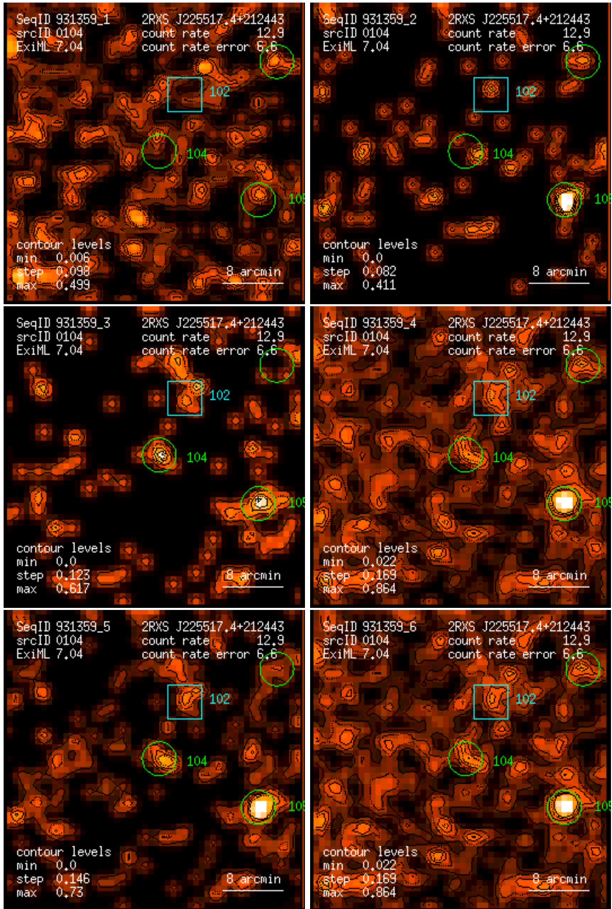
Figure 104: RASS 931359: detection 0104: band rate images, Gaussian filter: (1) PSPC channels 11 – 41, (2) 52 – 90, (3) 91 – 201, (4) 11 – 235, (5) 52 – 201, (6) 11 – 201. Broad band rates in counts/ks. Band rate contour levels in counts/ks/arcmin 2 .
