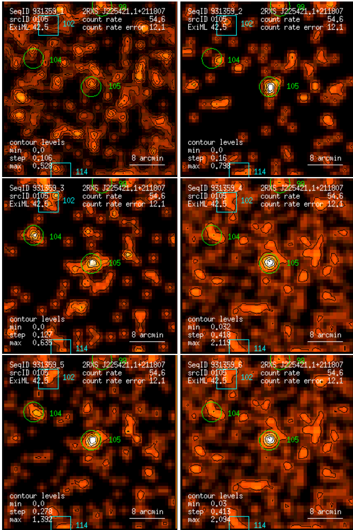
Figure 105: RASS 931359: detection 0105: band rate images, Gaussian filter: (1) PSPC channels 11 – 41, (2) 52 – 90, (3) 91 – 201, (4) 11 – 235, (5) 52 – 201, (6) 11 – 201. Broad band rates in counts/ks. Band rate contour levels in counts/ks/arcmin 2 .
