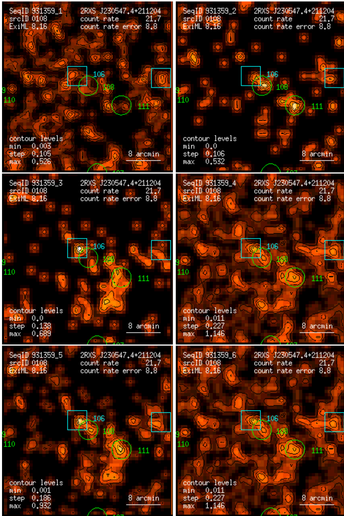
Figure 108: RASS 931359: detection 0108: band rate images, Gaussian filter: (1) PSPC channels 11 – 41, (2) 52 – 90, (3) 91 – 201, (4) 11 – 235, (5) 52 – 201, (6) 11 – 201. Broad band rates in counts/ks. Band rate contour levels in counts/ks/arcmin 2 .
