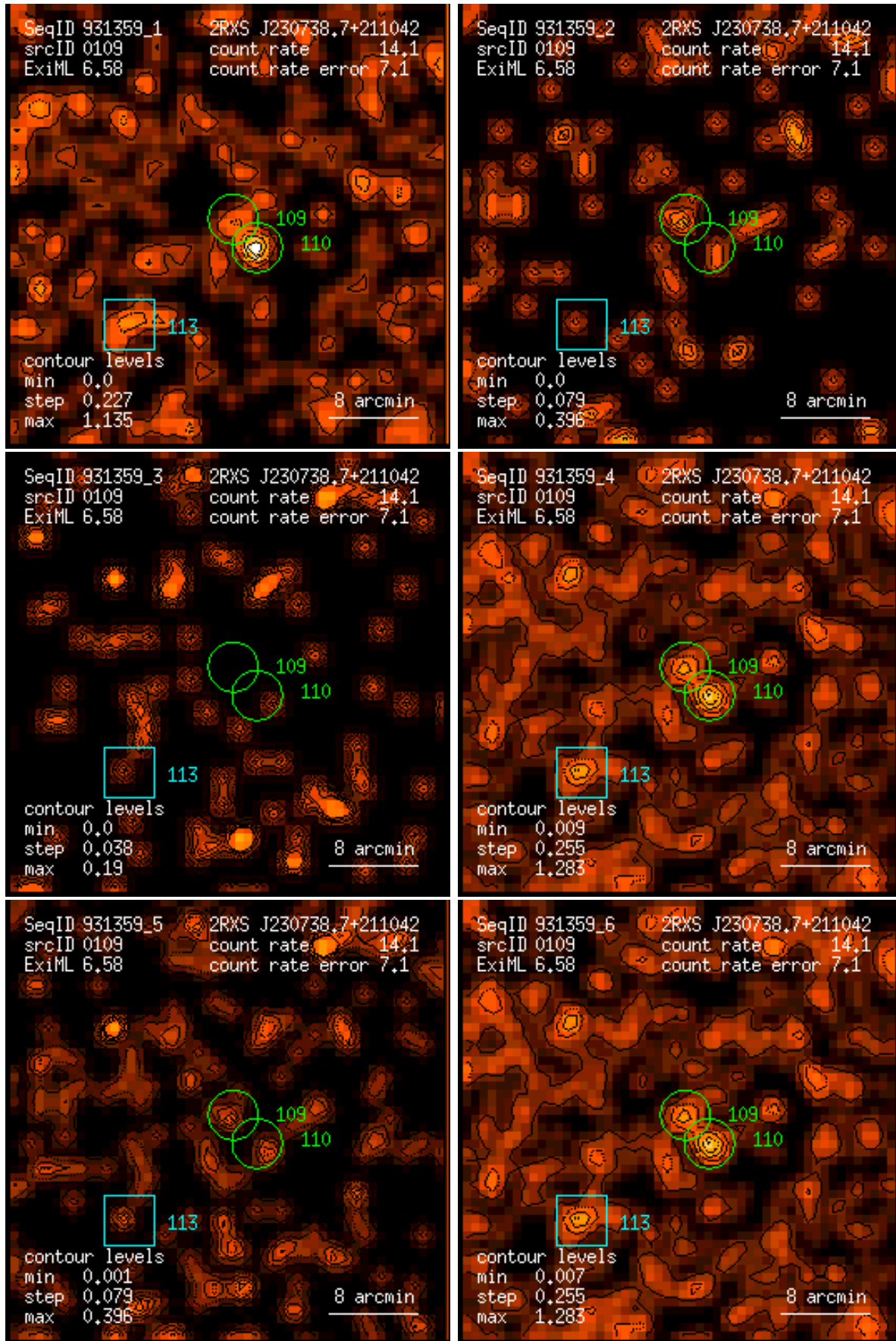
Figure 109: RASS 931359: detection 0109: band rate images, Gaussian filter: (1) PSPC channels 11 – 41, (2) 52 – 90, (3) 91 – 201, (4) 11 – 235, (5) 52 – 201, (6) 11 – 201. Broad band rates in counts/ks. Band rate contour levels in counts/ks/arcmin 2 .
