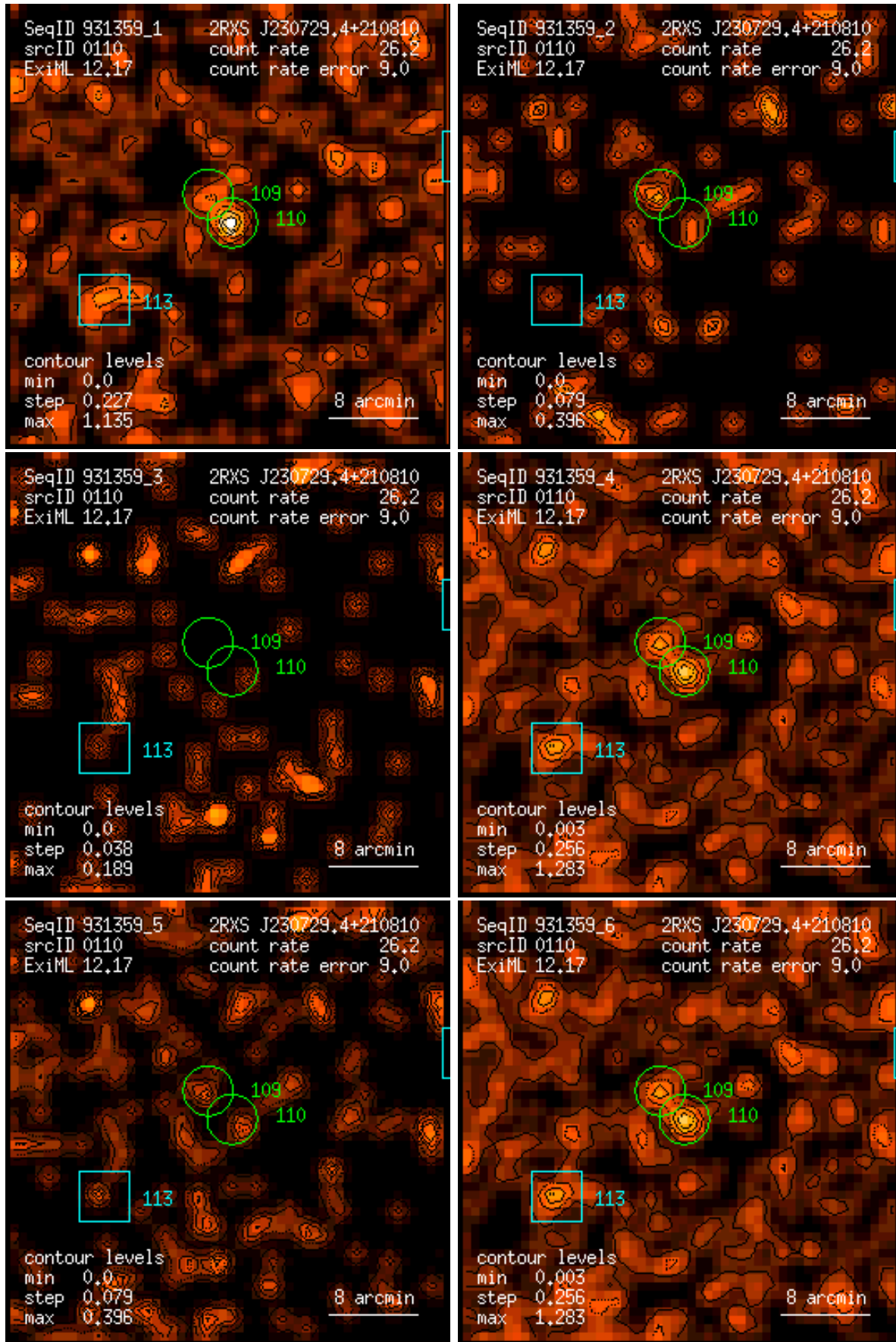
Figure 110: RASS 931359: detection 0110: band rate images, Gaussian filter: (1) PSPC channels 11 – 41, (2) 52 – 90, (3) 91 – 201, (4) 11 – 235, (5) 52 – 201, (6) 11 – 201. Broad band rates in counts/ks. Band rate contour levels in counts/ks/arcmin 2 .
