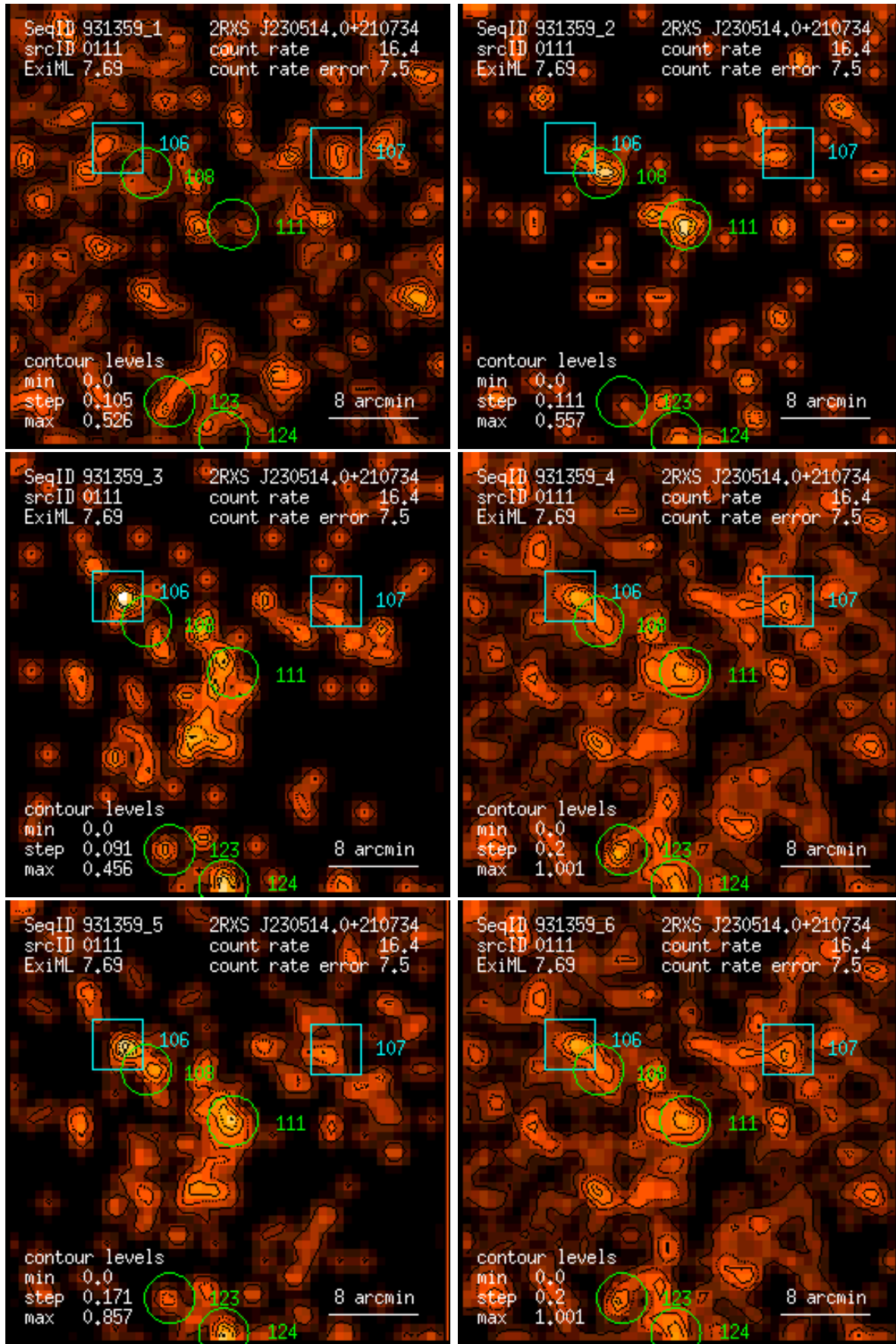
Figure 111: RASS 931359: detection 0111: band rate images, Gaussian filter: (1) PSPC channels 11 – 41, (2) 52 – 90, (3) 91 – 201, (4) 11 – 235, (5) 52 – 201, (6) 11 – 201. Broad band rates in counts/ks. Band rate contour levels in counts/ks/arcmin 2 .
