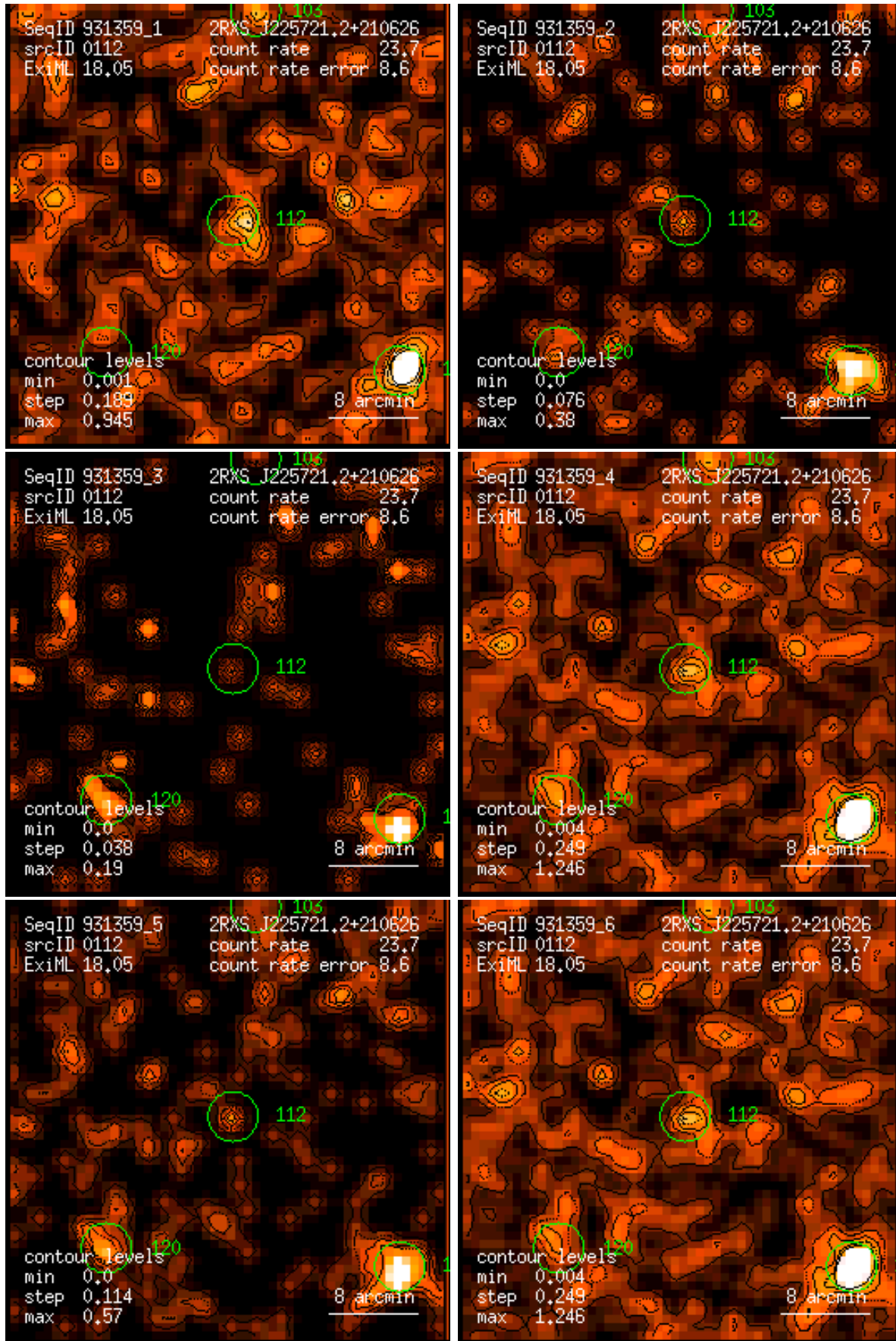
Figure 112: RASS 931359: detection 0112: band rate images, Gaussian filter: (1) PSPC channels 11 – 41, (2) 52 – 90, (3) 91 – 201, (4) 11 – 235, (5) 52 – 201, (6) 11 – 201. Broad band rates in counts/ks. Band rate contour levels in counts/ks/arcmin 2 .
