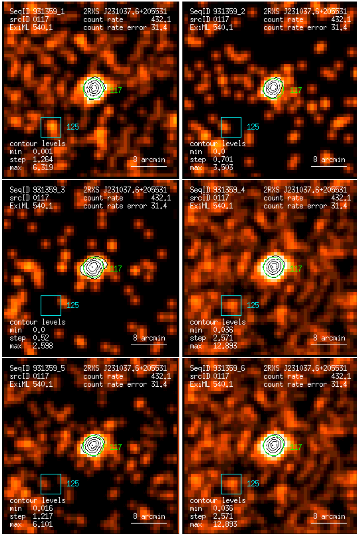
Figure 117: RASS 931359: detection 0117: band rate images, Gaussian filter: (1) PSPC channels 11 – 41, (2) 52 – 90, (3) 91 – 201, (4) 11 – 235, (5) 52 – 201, (6) 11 – 201. Broad band rates in counts/ks. Band rate contour levels in counts/ks/arcmin 2 .
