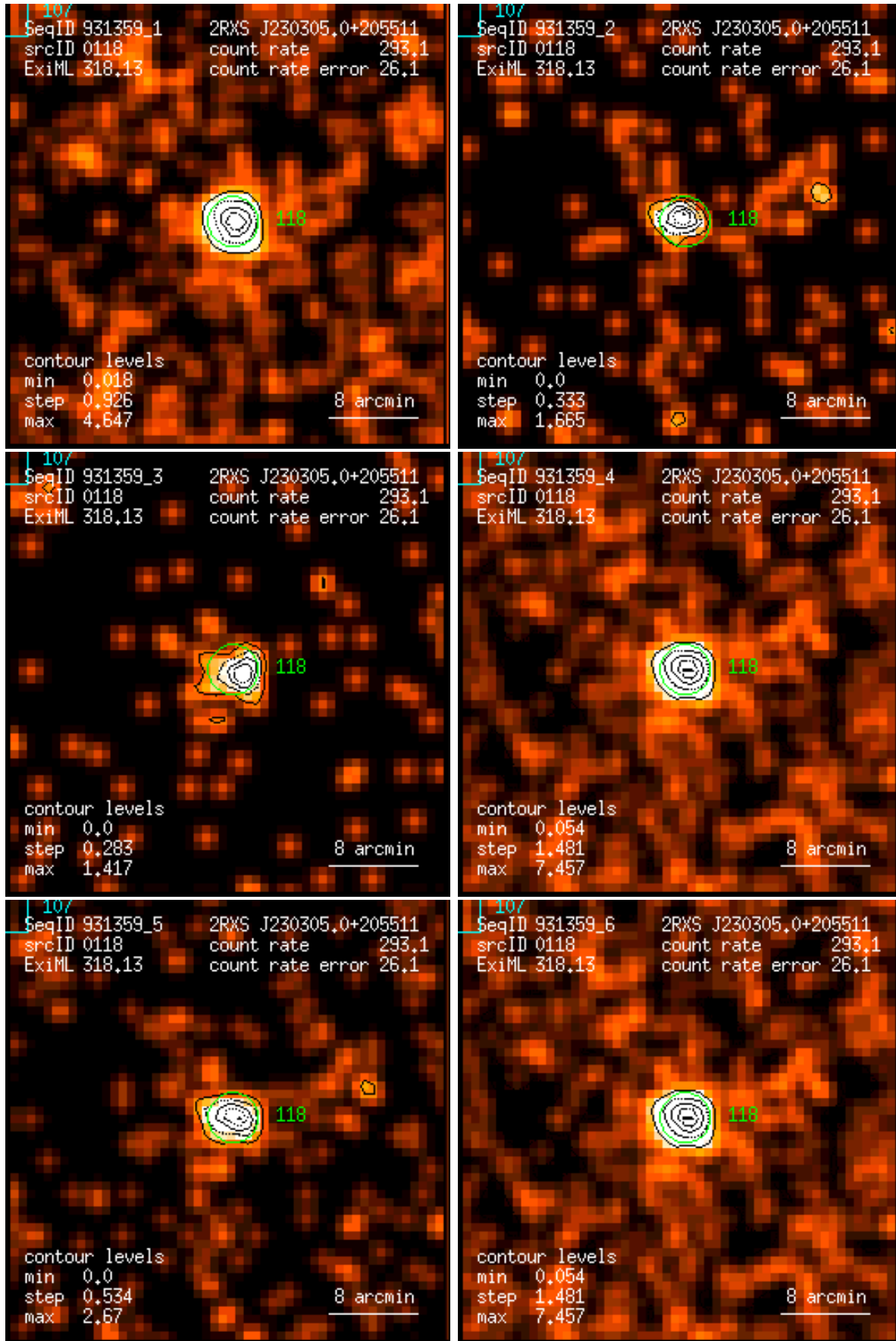
Figure 118: RASS 931359: detection 0118: band rate images, Gaussian filter: (1) PSPC channels 11 – 41, (2) 52 – 90, (3) 91 – 201, (4) 11 – 235, (5) 52 – 201, (6) 11 – 201. Broad band rates in counts/ks. Band rate contour levels in counts/ks/arcmin 2 .
