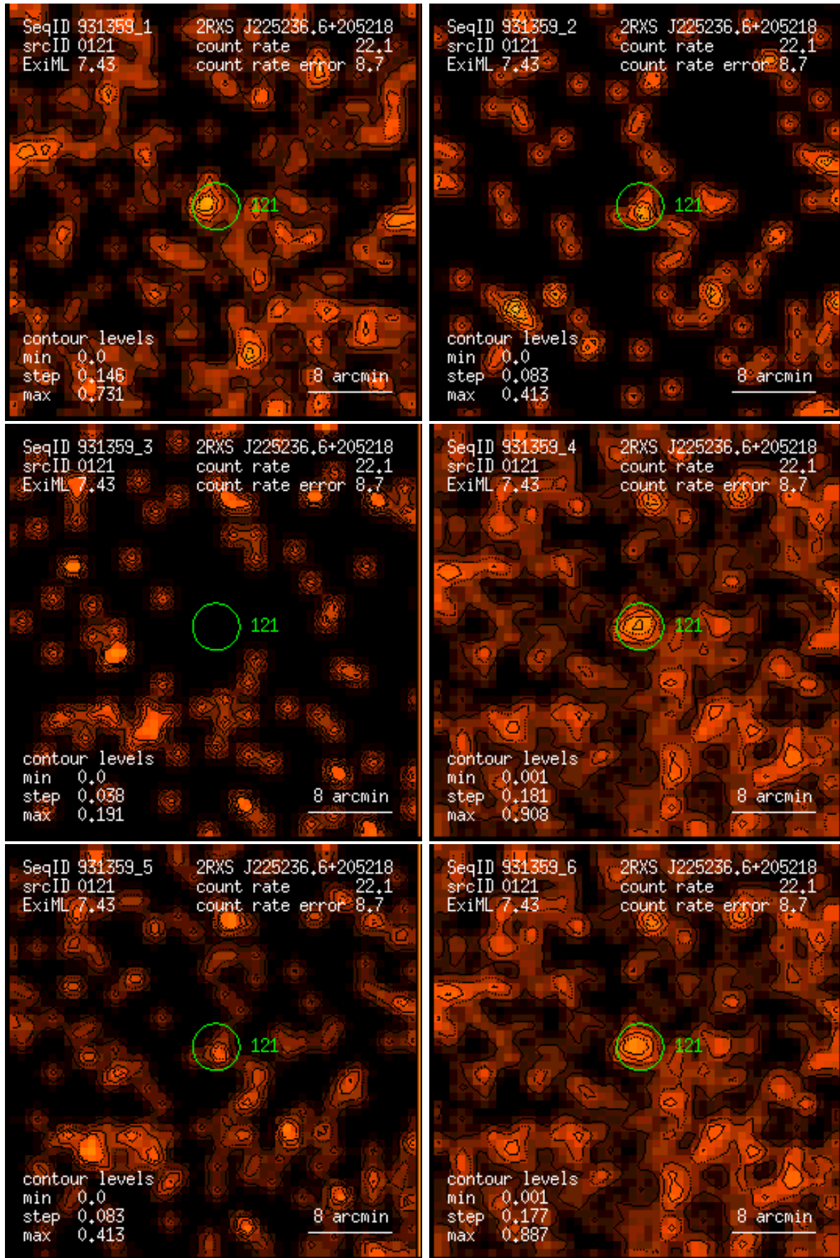
Figure 121: RASS 931359: detection 0121: band rate images, Gaussian filter: (1) PSPC channels 11 – 41, (2) 52 – 90, (3) 91 – 201, (4) 11 – 235, (5) 52 – 201, (6) 11 – 201. Broad band rates in counts/ks. Band rate contour levels in counts/ks/arcmin 2 .
