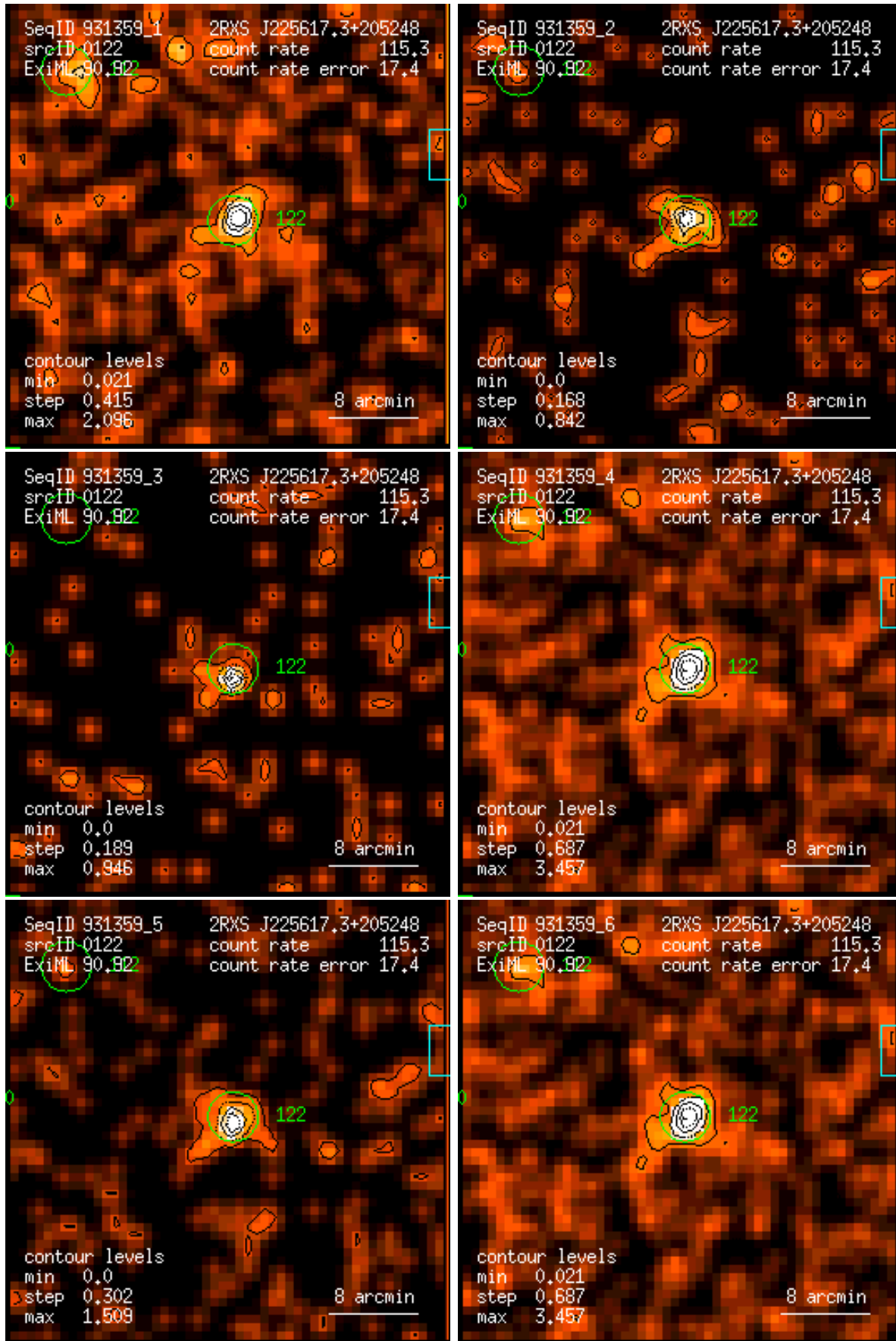
Figure 122: RASS 931359: detection 0122: band rate images, Gaussian filter: (1) PSPC channels 11 – 41, (2) 52 – 90, (3) 91 – 201, (4) 11 – 235, (5) 52 – 201, (6) 11 – 201. Broad band rates in counts/ks. Band rate contour levels in counts/ks/arcmin 2 .
