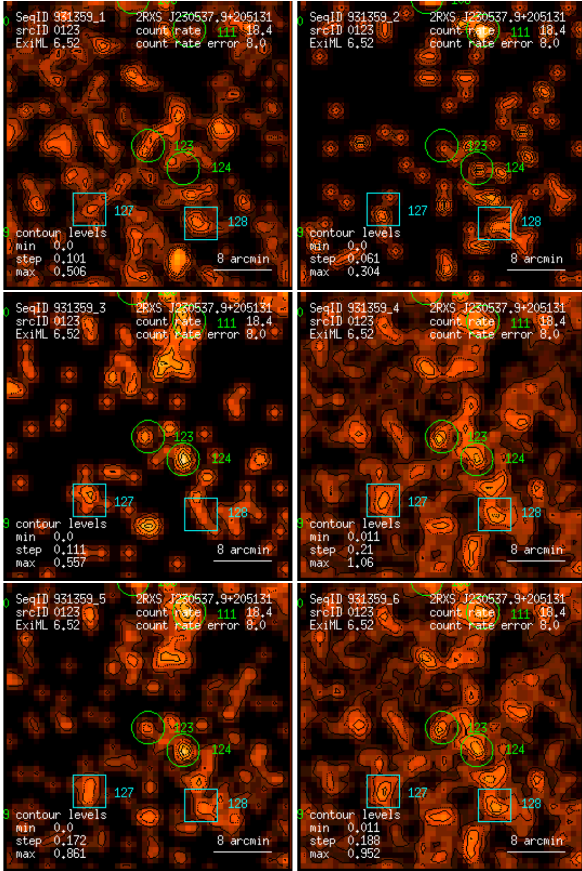
Figure 123: RASS 931359: detection 0123: band rate images, Gaussian filter: (1) PSPC channels 11 – 41, (2) 52 – 90, (3) 91 – 201, (4) 11 – 235, (5) 52 – 201, (6) 11 – 201. Broad band rates in counts/ks. Band rate contour levels in counts/ks/arcmin 2 .
