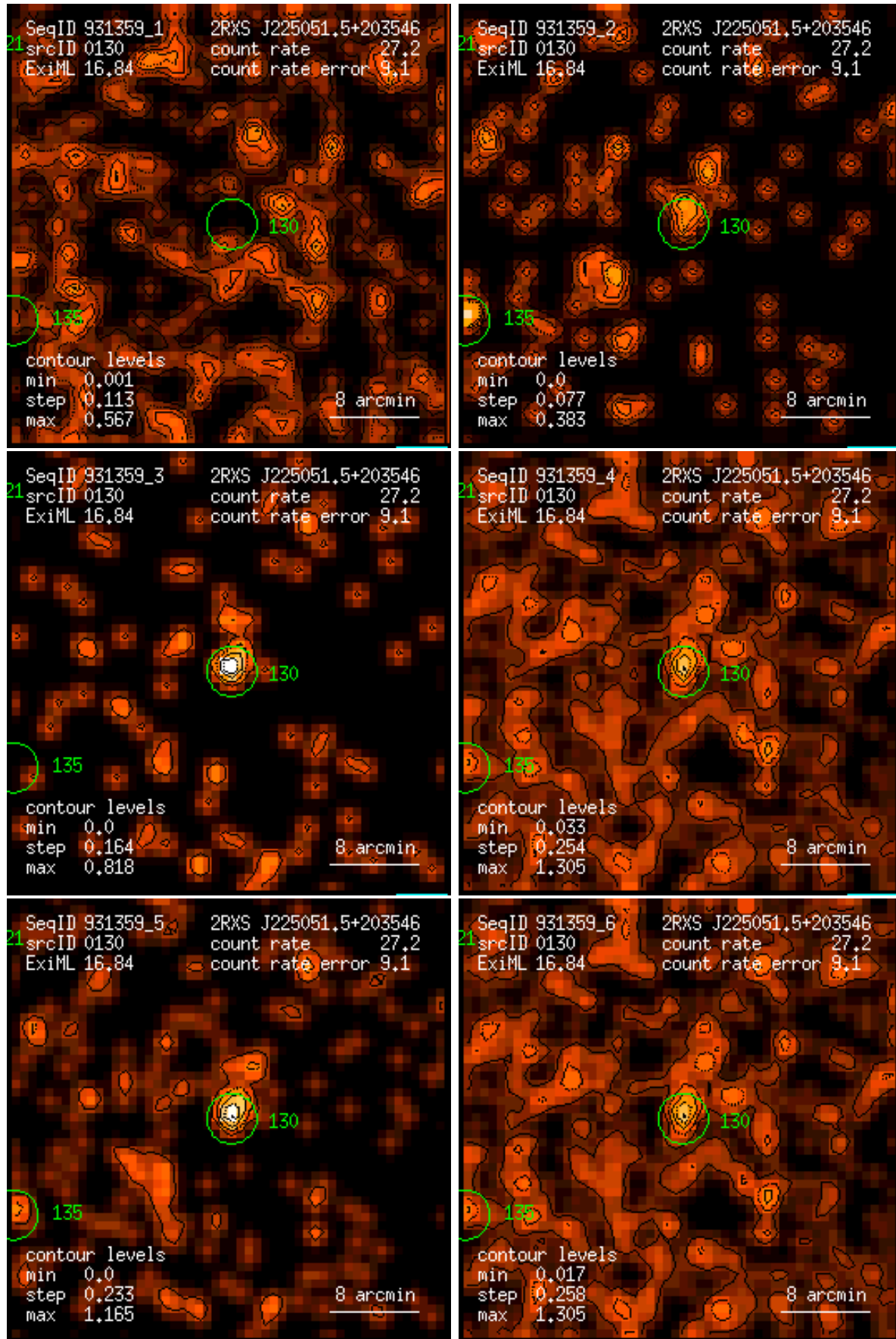
Figure 130: RASS 931359: detection 0130: band rate images, Gaussian filter: (1) PSPC channels 11 – 41, (2) 52 – 90, (3) 91 – 201, (4) 11 – 235, (5) 52 – 201, (6) 11 – 201. Broad band rates in counts/ks. Band rate contour levels in counts/ks/arcmin 2 .
