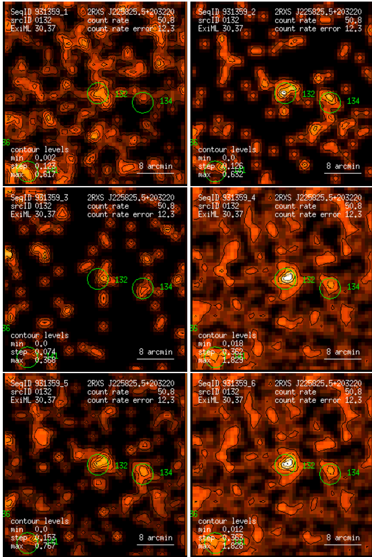
Figure 132: RASS 931359: detection 0132: band rate images, Gaussian filter: (1) PSPC channels 11 – 41, (2) 52 – 90, (3) 91 – 201, (4) 11 – 235, (5) 52 – 201, (6) 11 – 201. Broad band rates in counts/ks. Band rate contour levels in counts/ks/arcmin 2 .
