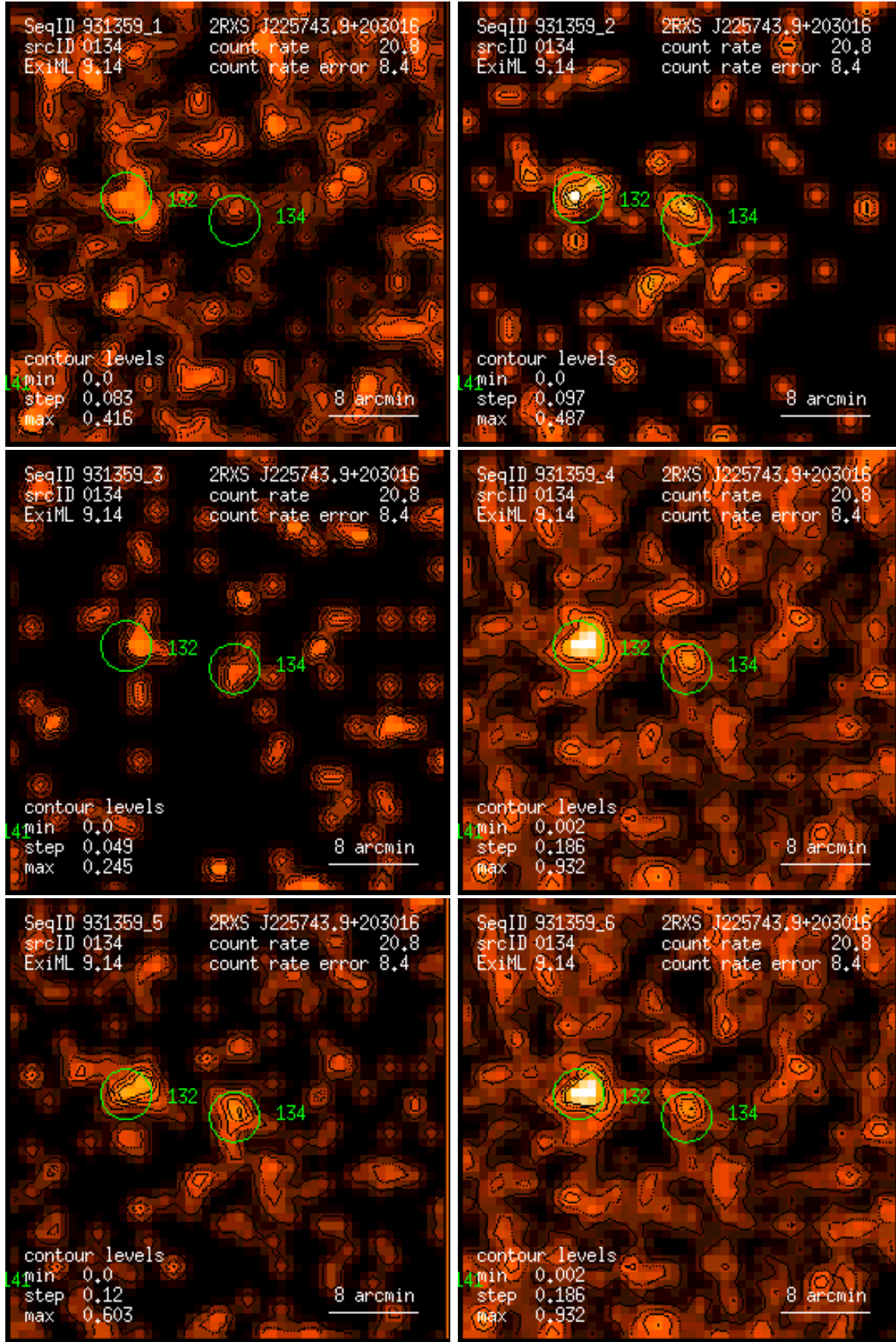
Figure 134: RASS 931359: detection 0134: band rate images, Gaussian filter: (1) PSPC channels 11 – 41, (2) 52 – 90, (3) 91 – 201, (4) 11 – 235, (5) 52 – 201, (6) 11 – 201. Broad band rates in counts/ks. Band rate contour levels in counts/ks/arcmin 2 .
