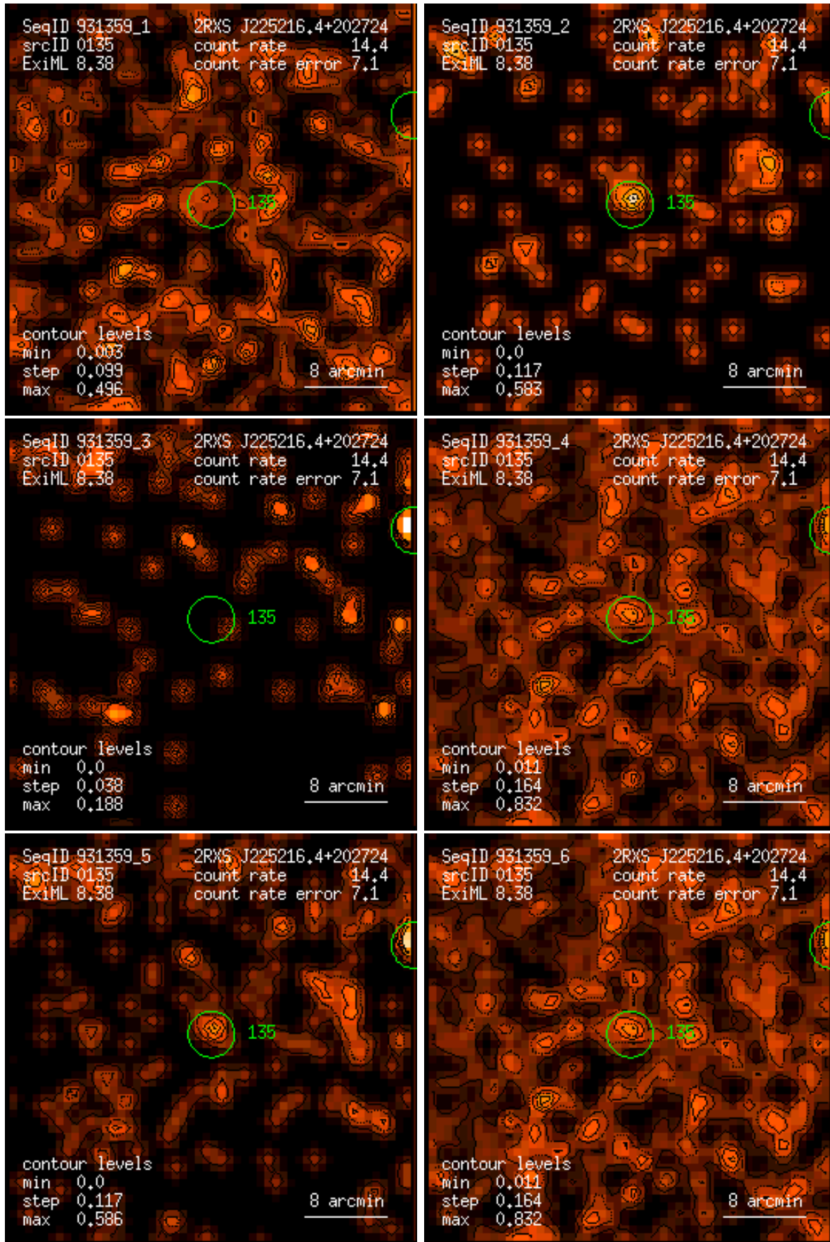
Figure 135: RASS 931359: detection 0135: band rate images, Gaussian filter: (1) PSPC channels 11 – 41, (2) 52 – 90, (3) 91 – 201, (4) 11 – 235, (5) 52 – 201, (6) 11 – 201. Broad band rates in counts/ks. Band rate contour levels in counts/ks/arcmin 2 .
